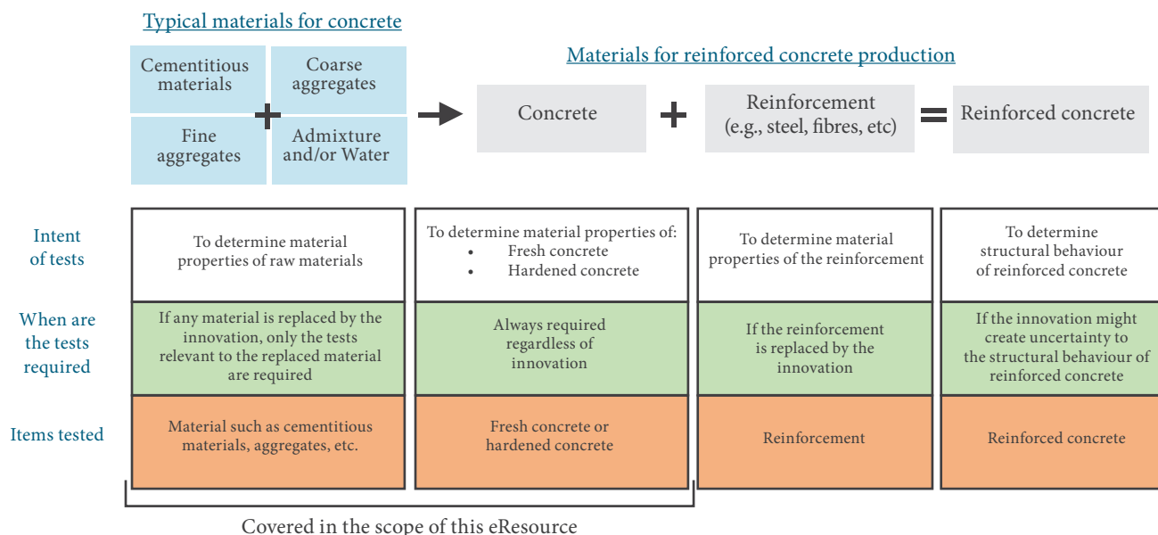
Figure 3.1: Composition of concrete, intent of different tests, and the need for such tests
