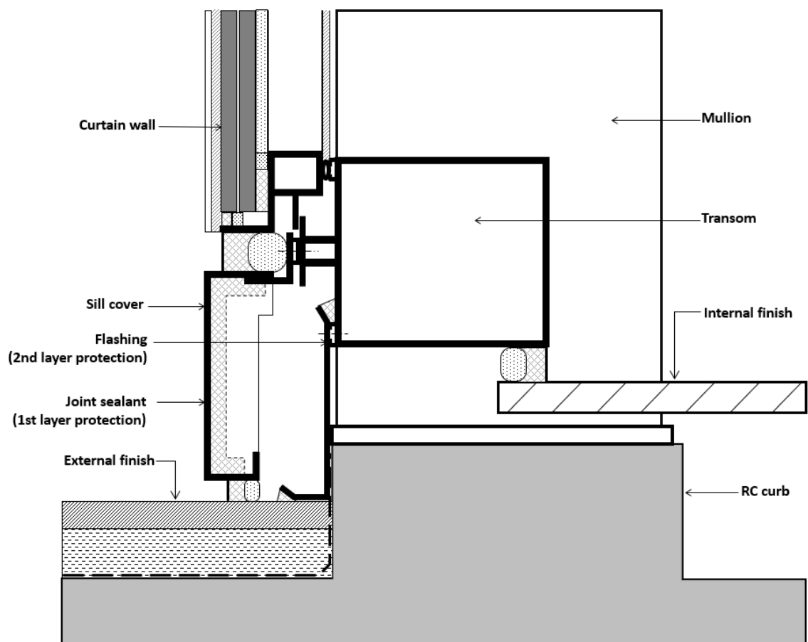
Figure 11: Drawing illustrating double layer protection at bottom flashing, in this case sealant (1 st layer of protection) and flashing (2 nd layer of protection).
