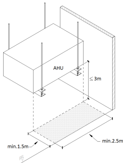
Figure 38: Ground clearance to mount scaffold for AHU located \leq 3\text{ m}
