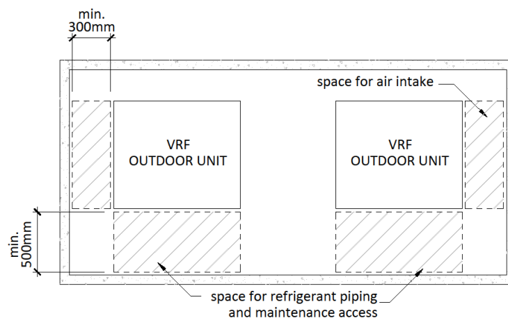
Figure 214 Space requirement for VRF outdoor installation (top discharge) – top view
