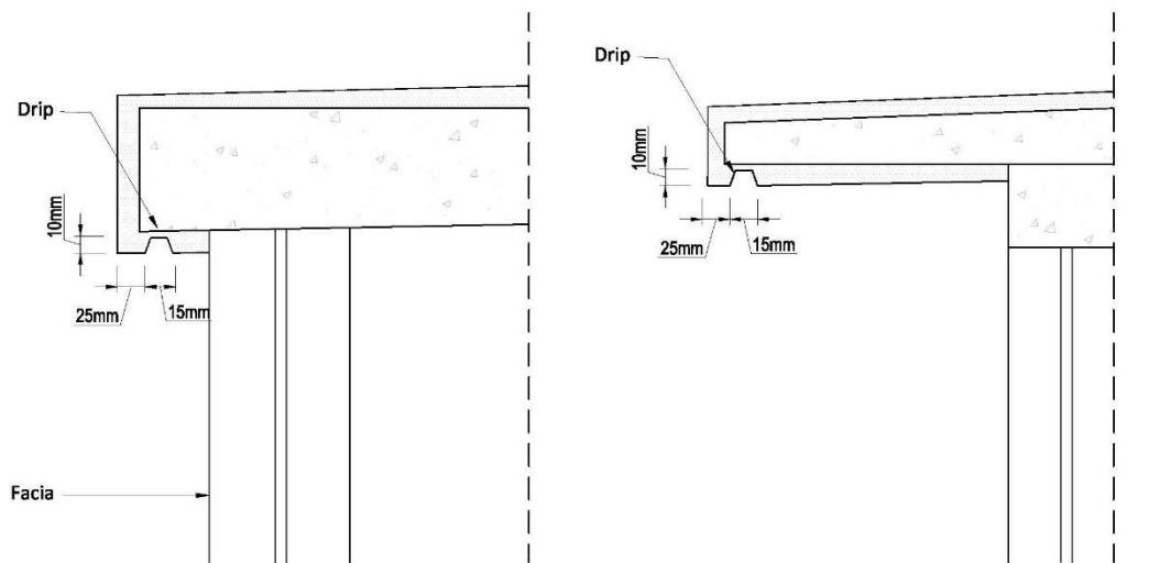
Figure 2: Typical drip edge detail on projected façade elements. Image on the left illustrates detail on recessed window and image on right illustrates detail on sunshades.
