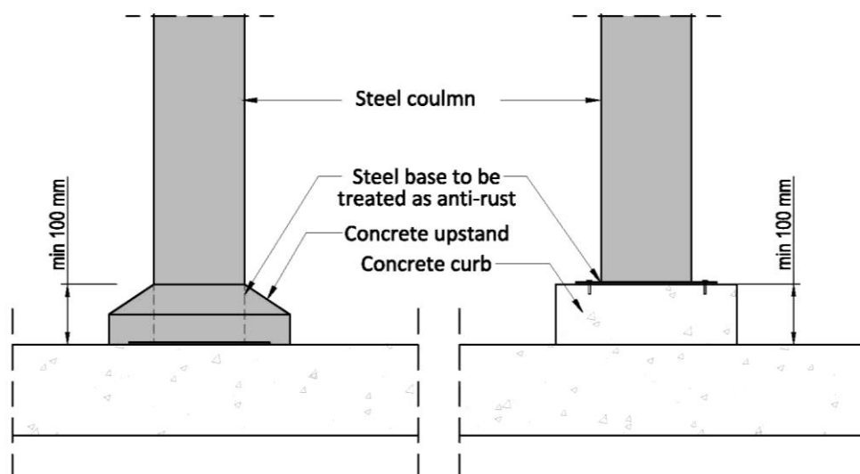
Figure 60 - Concrete upstand protection for steel base
