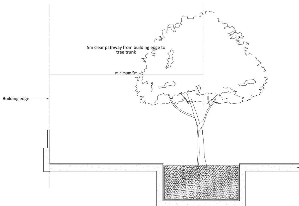
Figure 58 - Typical section showing buffer zone required for trees
