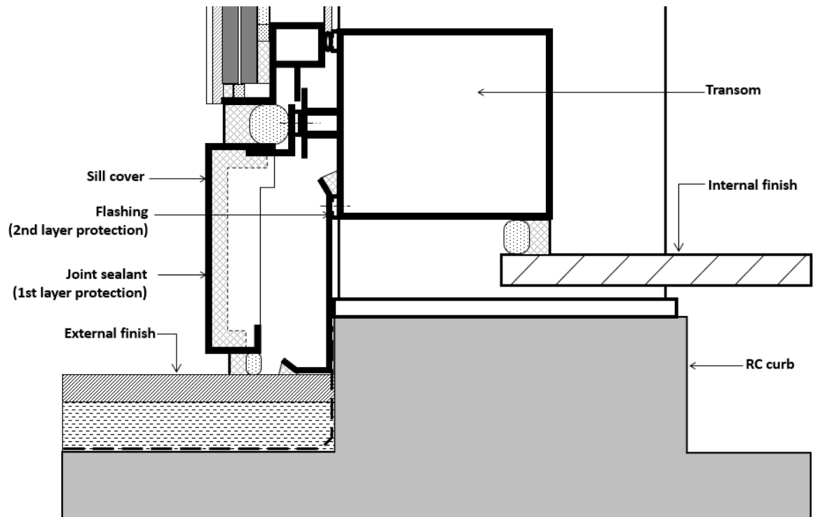
Figure 8: Drawing illustrating double layer protection at bottom flashing, in this case sealant (1 st layer of protection) and flashing (2 nd layer of protection).
