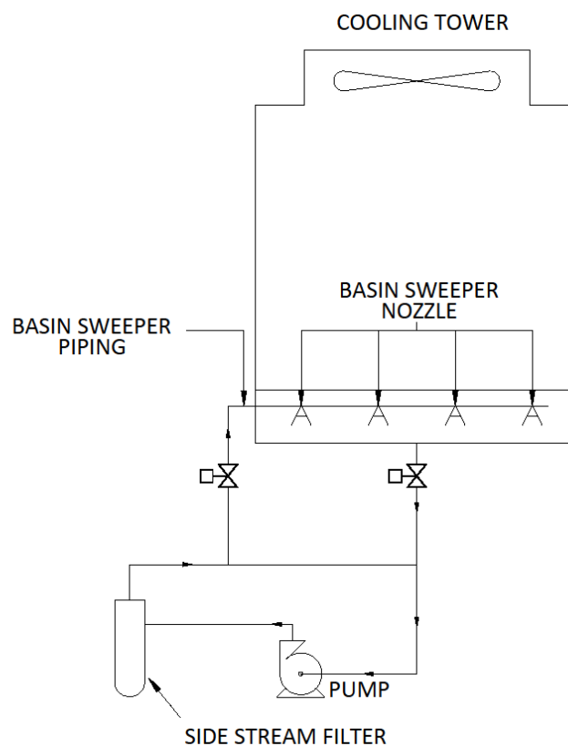
Figure 29: Cooling tower basin sweeper system
