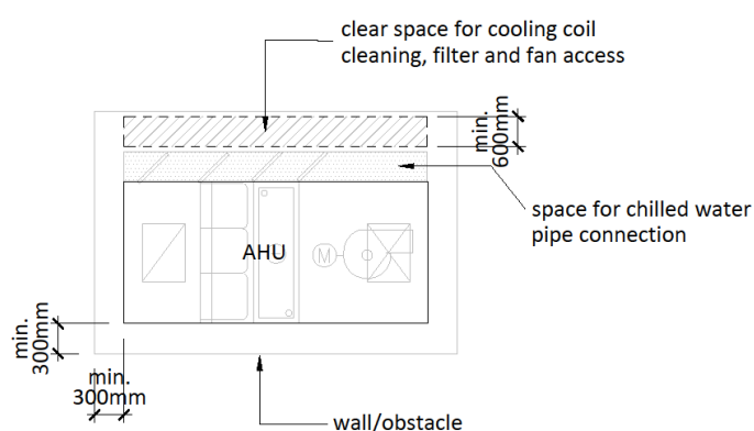
Figure 37: Typical access provision for ceiling suspended AHU
