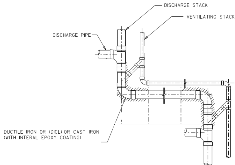
Figure 47: Hubless elbows for sanitary stacks with horizontal transfers
