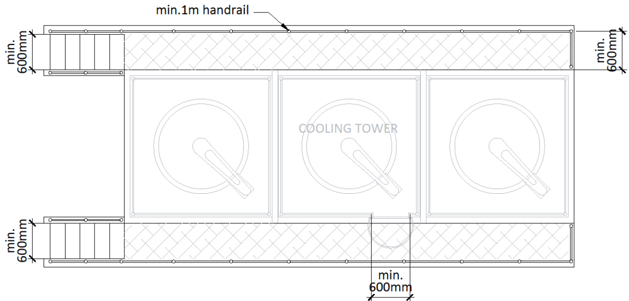
Figure 112: Cooling tower with catwalk (2 sides)
