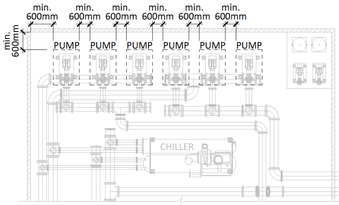
Figure 89: Access space requirement for pump (part plan)
