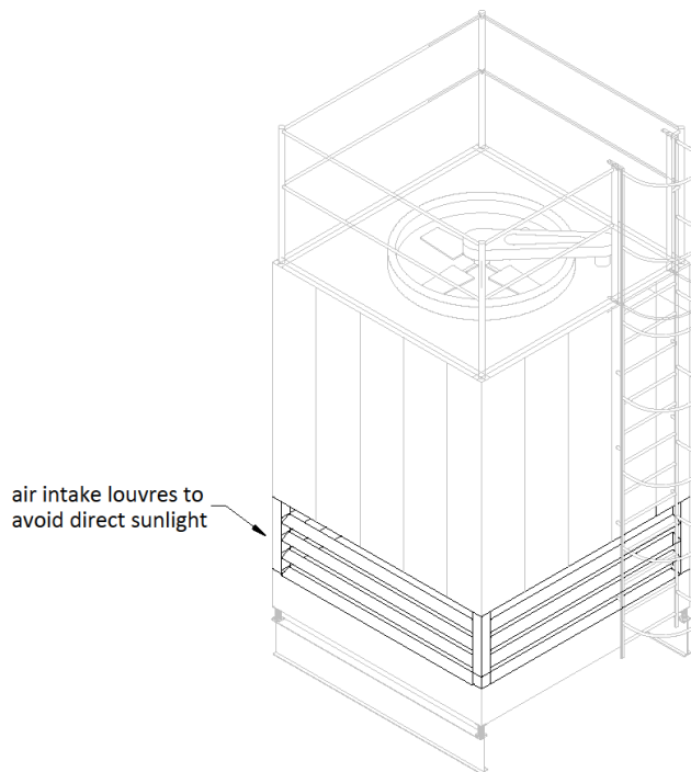
Figure 27: Counter flow cooling tower with air intake louvres
