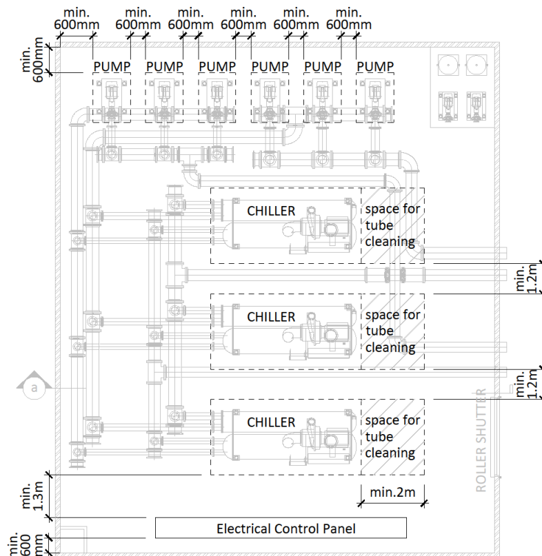
Figure 16: Typical chiller plant room layout and space provision
