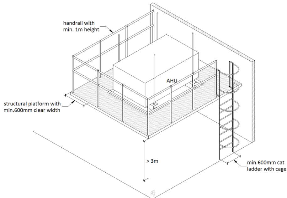
Figure 39: Cat ladder with structural platform to access AHU located > 3\text{ m}
