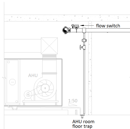
Figure 48: Flow switch drain valve in rooms with floor trap
