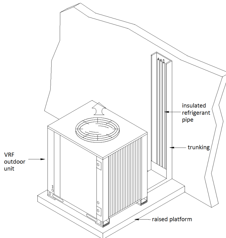
Figure 225: Trucking for refrigerant pipe
