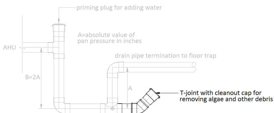
Figure 242: Typical detail for AHU drain termination
