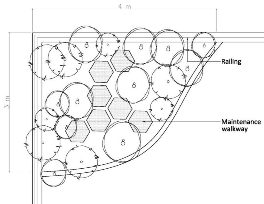
Figure 57 - Maintenance walkway for planter box more than 1m wide
