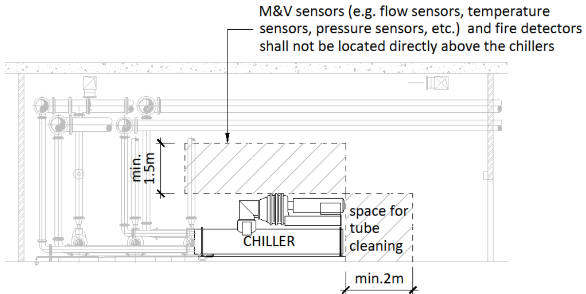
Figure 78: Headroom requirement for chiller
