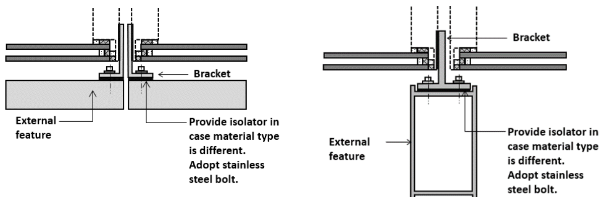
Figure 3: Example - plan drawing (detail) on left and right illustrating connection between curtain wall and metal external feature on the exposed face of the façade. Providing metals of similar metal properties or separator/isolator helps to mitigate risk of bi-metallic corrosion.
