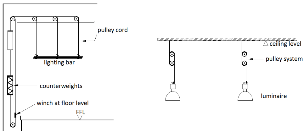
Figure 50: Group pulley system (left) and single pulley system (right)
