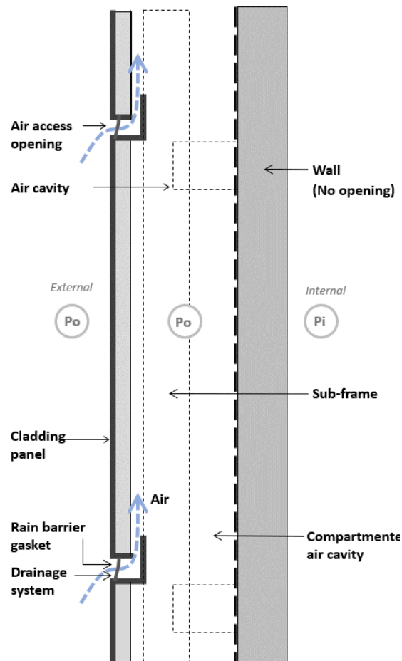
Figure 5: Drawing illustrating pressure equalised metal cladding system.
