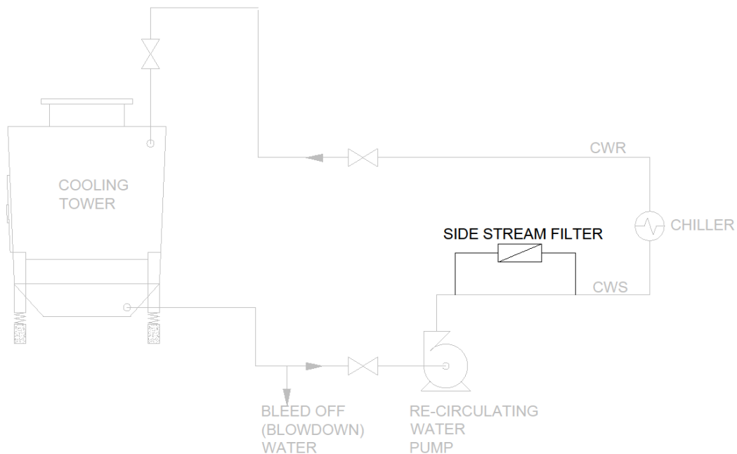
Figure 160: Schematic diagram for side stream filtration system
