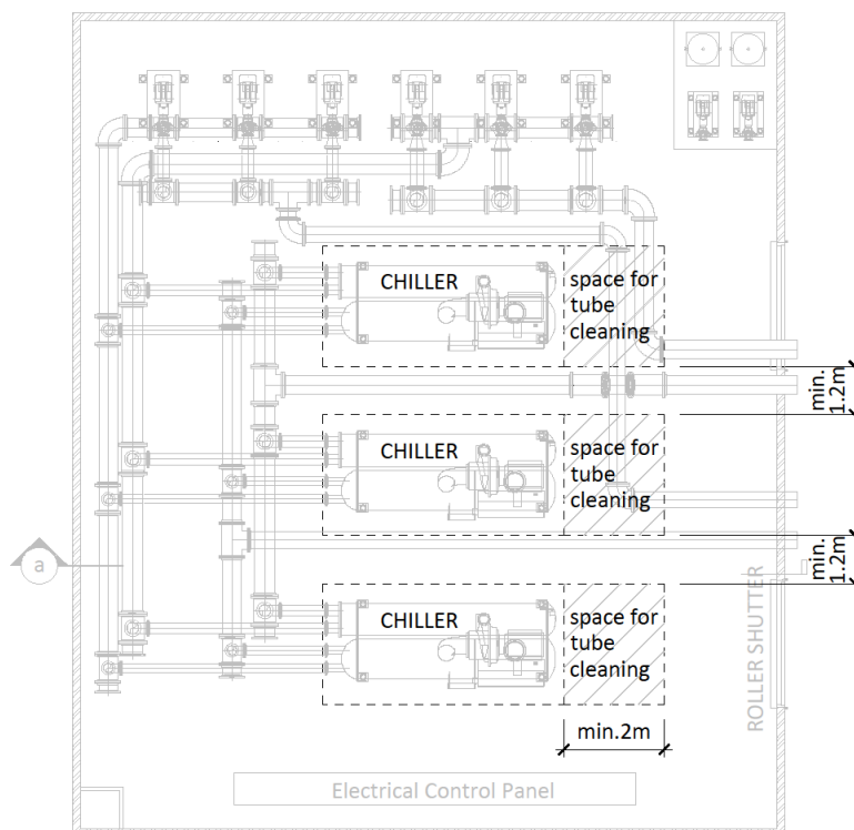
Figure 6: Access space for chiller
