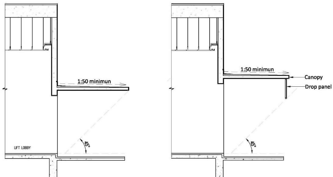
Figure 13 : Design of canopy overhang (left), Design of canopy overhang with drop panel (right)
