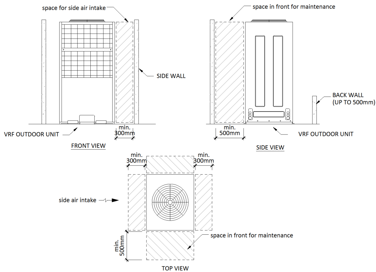
Figure 17: Space requirement for single VRF outdoor installation (top discharge)
