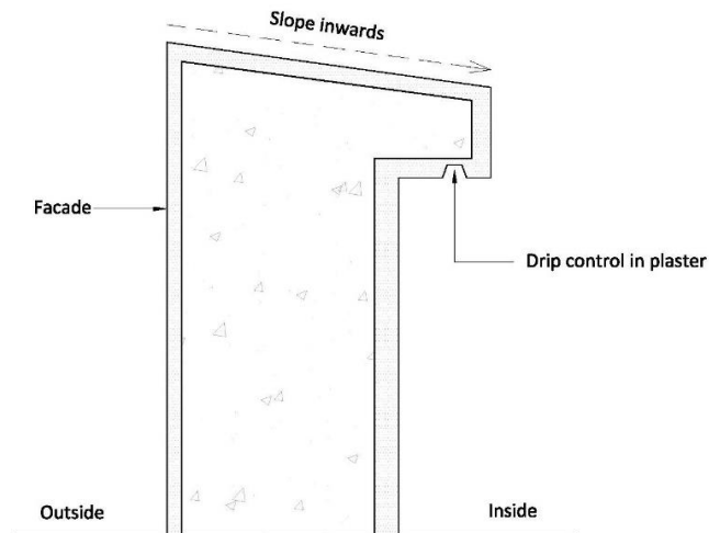
Figure 2: Drawing illustrating slope gradient on top surface of external wall.
