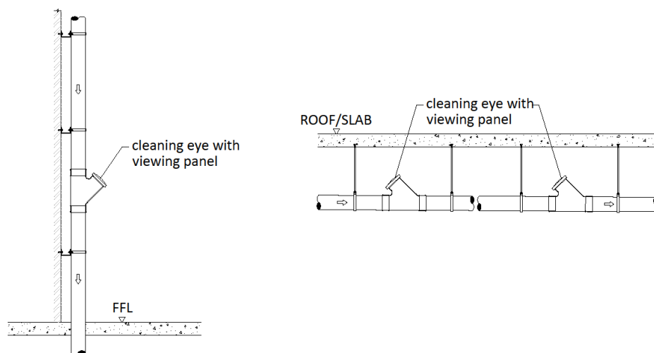
Figure 46: Sanitary pipe with cleaning eye that equipped with viewing panel
