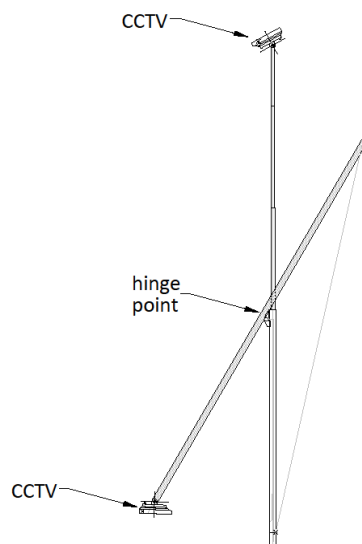
Figure 273: CCTV with foldable pole and arm
