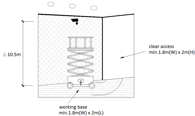
Figure 284: Clear access for CCTV with mounting height \leq 10.5\text{m}
