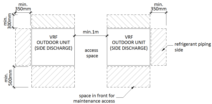
Figure 203: Space requirement for collective VRF outdoor unit (side discharge) - top view
