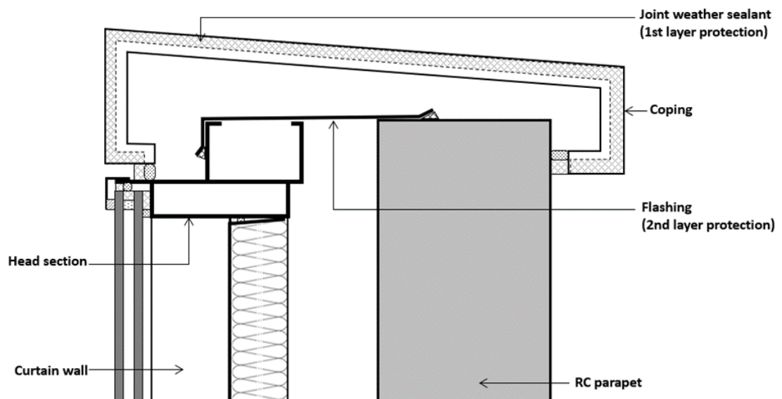
Figure 10: Drawing illustrating double layer protection at façade coping, in this case sealant (1 st layer of protection) and flashing (2 nd layer of protection).
