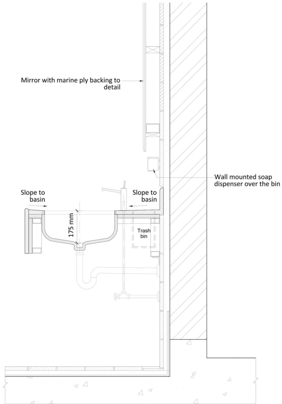
Figure 15- Schematic sectional drawing with vanity basin
