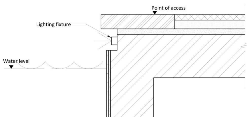
Figure 55 – Section showing example of lighting system located outside the water
