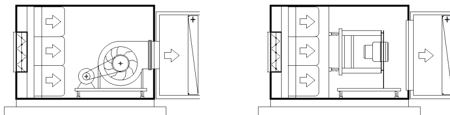
Figure 254: Conventional (left) and Direct Drive Fan system (right)
