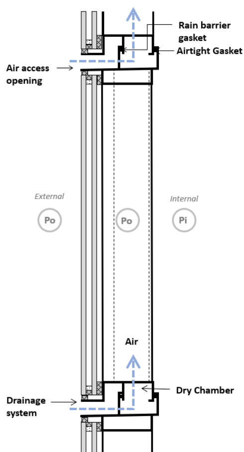
Figure 9: Drawing illustrating pressure equalised system.
