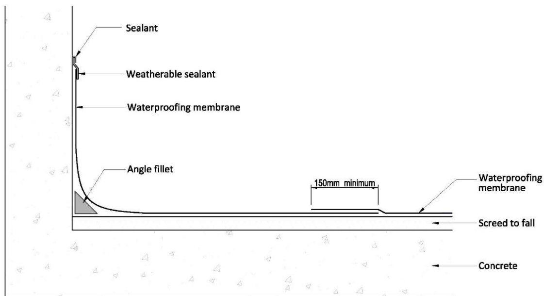
Figure 14 : waterproofing termination and overlapping detail
