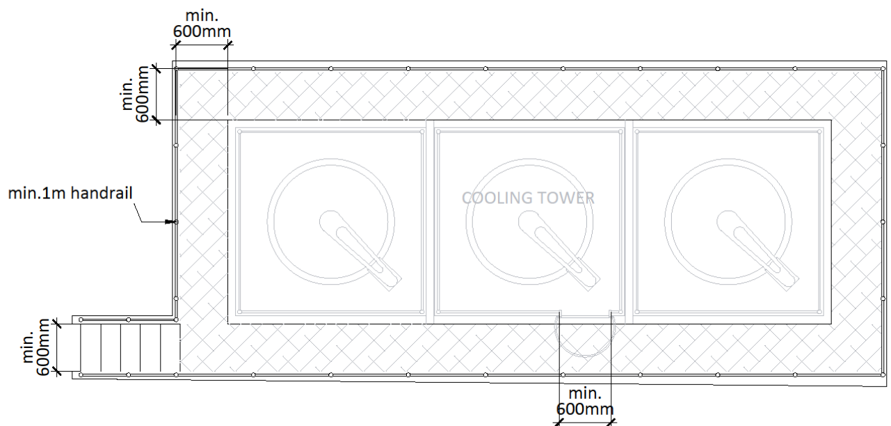
Figure 101: Cooling tower with catwalk (4 sides)
