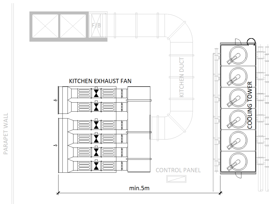
Figure 28: Roof with cooling tower and kitchen exhaust fan
