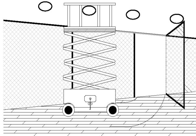
Figure 49: Clearance for MEWP
