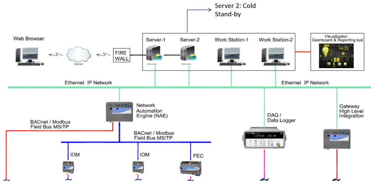
Typical BMS System Architecture with cold stand-by arrangement
