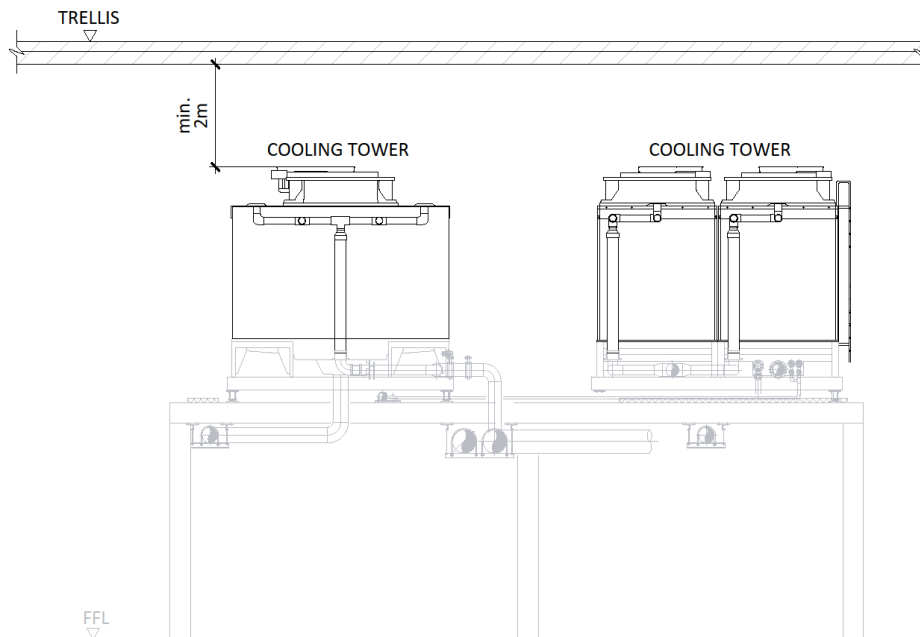
Figure 145: Headroom requirement for cooling tower with trellis
