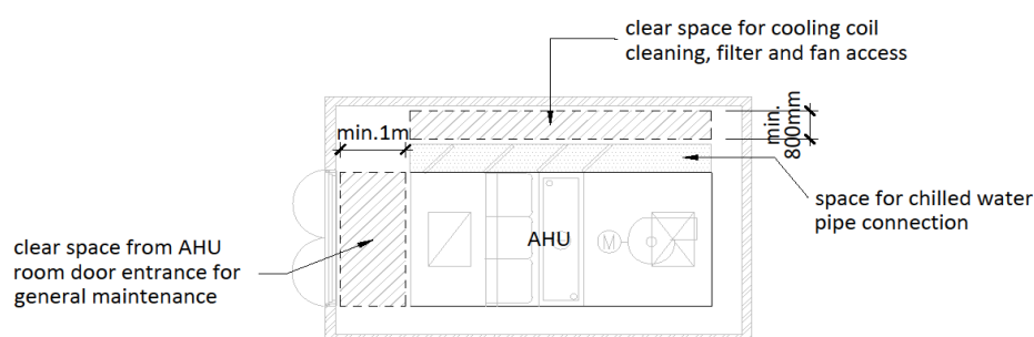
Figure 36: AHU room plan drawing
