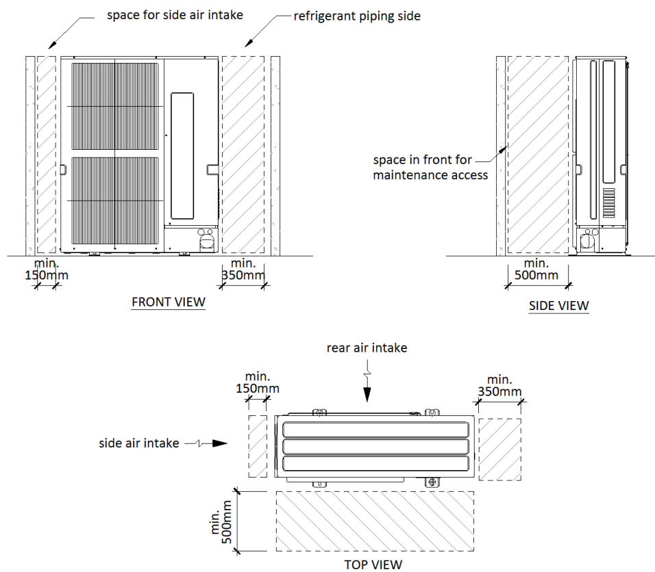
Figure 181: Space requirement for single VRF outdoor installation (side discharge)
