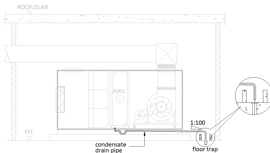
Figure 231: Typical AHU condensate drain termination
