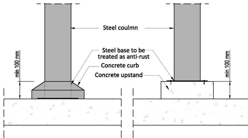
Figure 12: Concrete protection for steel base.
