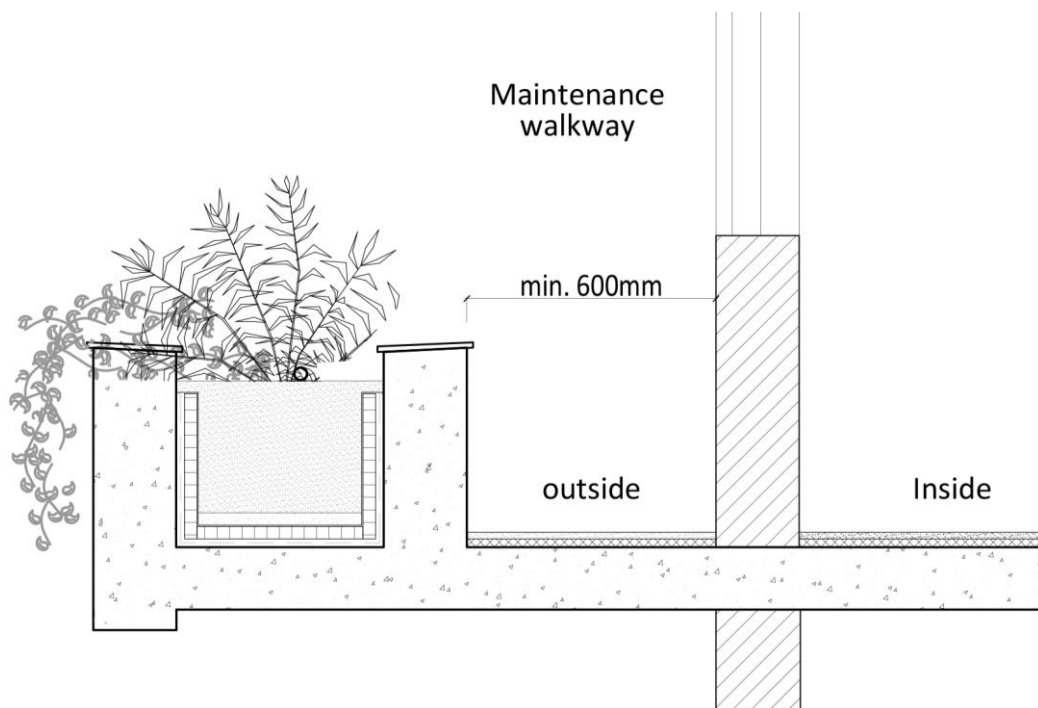
Figure 59- Planter box with maintenance walkway
