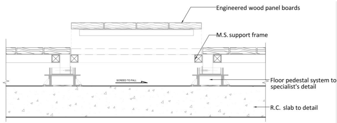
Figure 56 - Typical section showing demountable fixture deck system
