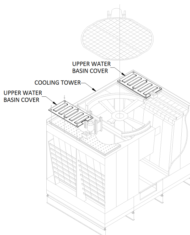
Figure 156: Cross flow cooling tower with upper water basin cover
