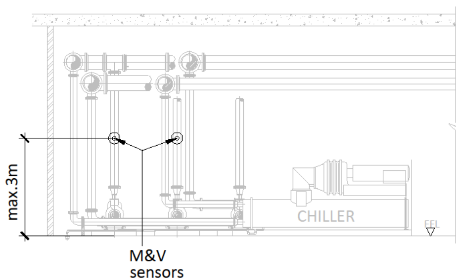
Figure 9: Location requirement for M&V sensors (part plan)
