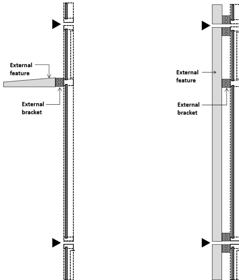
Figure 4: Example - section drawing (detail) on left and right illustrating connection between curtain wall and metal external feature on the exposed face of the facade. Providing metals of similar metal properties or separator/isolator helps to mitigate risk of bi-metallic corrosion.
