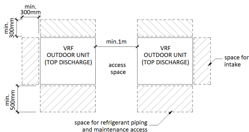
Figure 192: Space requirement for collective VRF outdoor unit (top discharge) – top view
