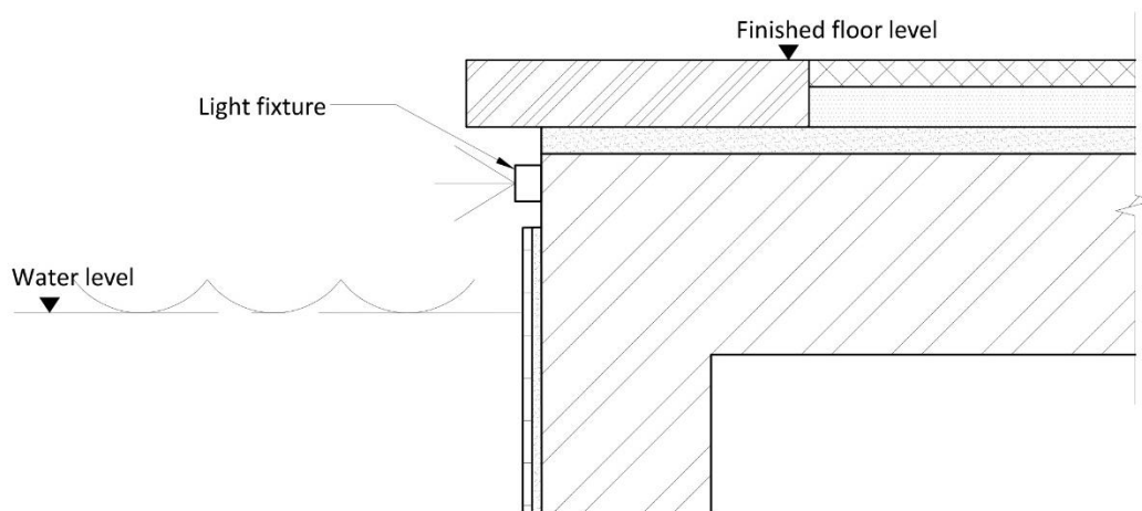
Figure 26 - Example of lighting system located above the water
