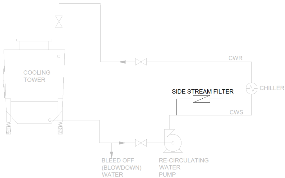
Figure 110: Schematic diagram for side stream filtration system
