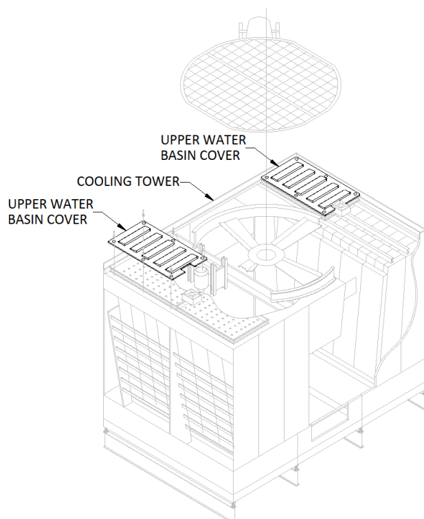
Figure 26: Cross flow cooling tower with upper water basin cover
