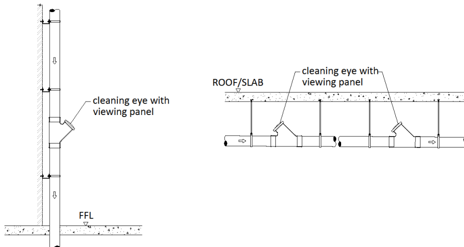
Figure 21: Sanitary pipe with cleaning eye that equipped with viewing panel
