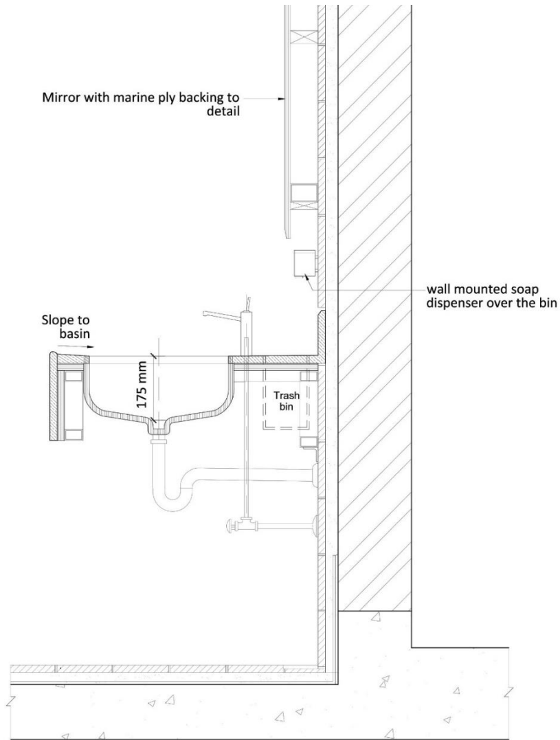
Figure 17 - Schematic sectional drawing with vanity basin
