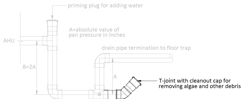
Figure 39: Typical detail for AHU drain termination
