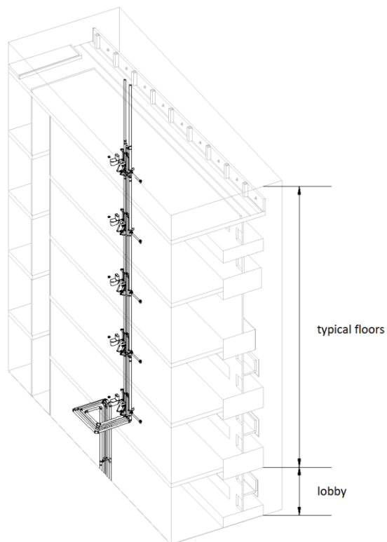
Figure 22: Risers with continuous vertical run without any offsets for typical floors
