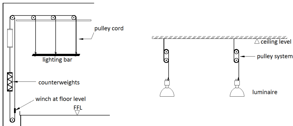
Figure 48: Group pulley system (left) and single pulley system (right)
