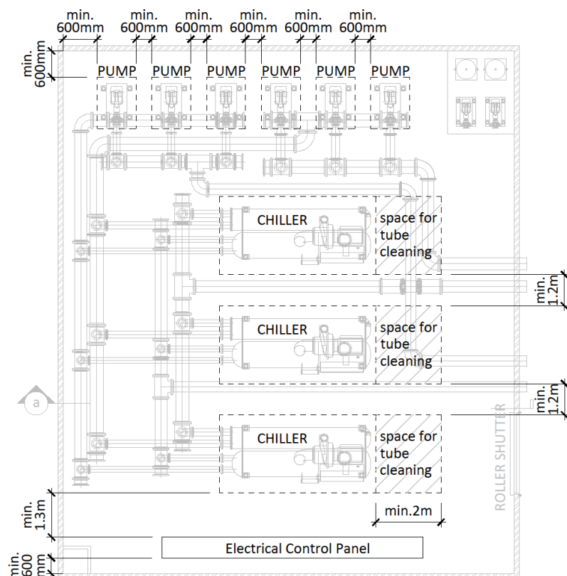
Figure 19: Typical chiller plant room layout and space provision
