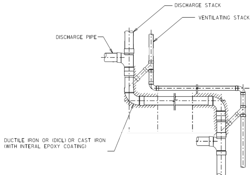
Figure 44: Hubless elbows for sanitary stacks with horizontal transfers 27
