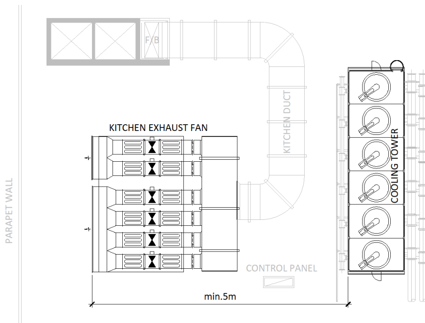
Figure 28: Roof with cooling tower and kitchen exhaust fan
