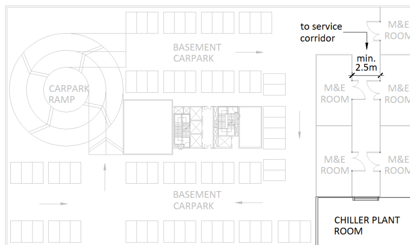
Figure 71: Basement chiller plant with service corridor
