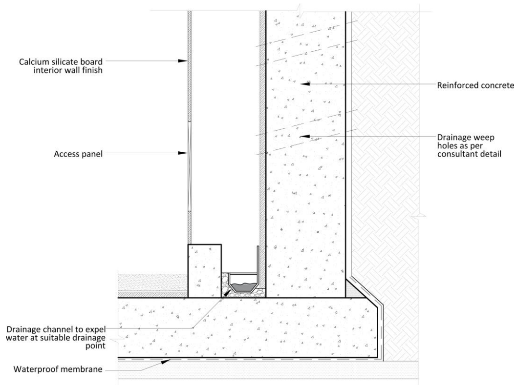
Figure 18 - Typical section of cavity wall with waterproofing
