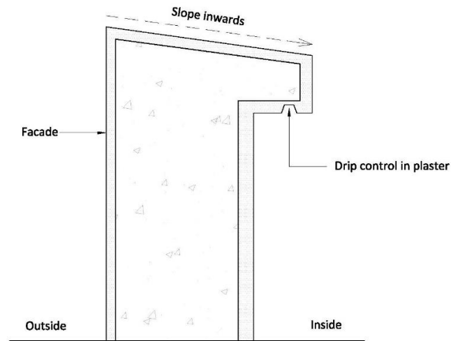
Figure 3: Drawing illustrating slope gradient on top surface of external wall.
