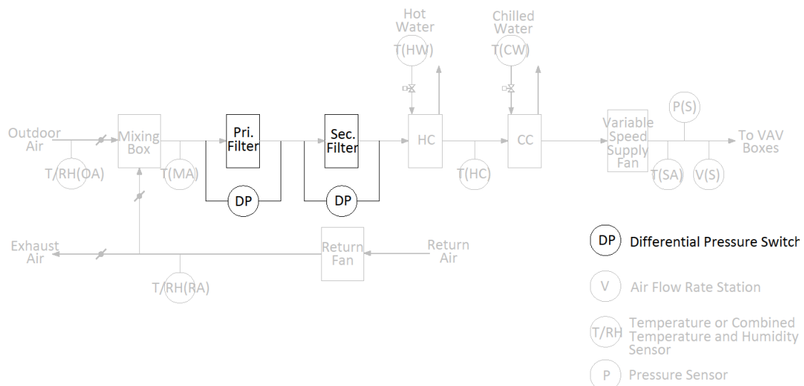
Figure 19: AHU diagram showing the differential pressure switch
