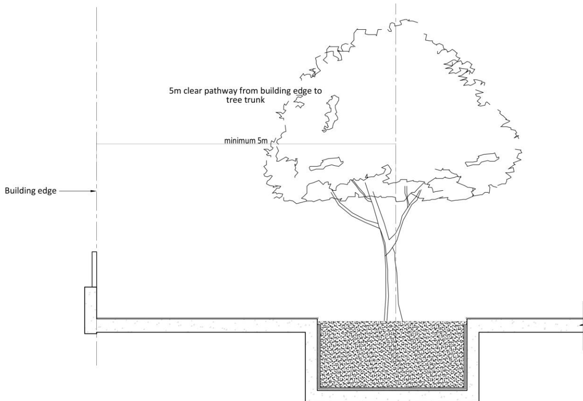
Figure 30 - Typical section showing buffer zone required for trees
