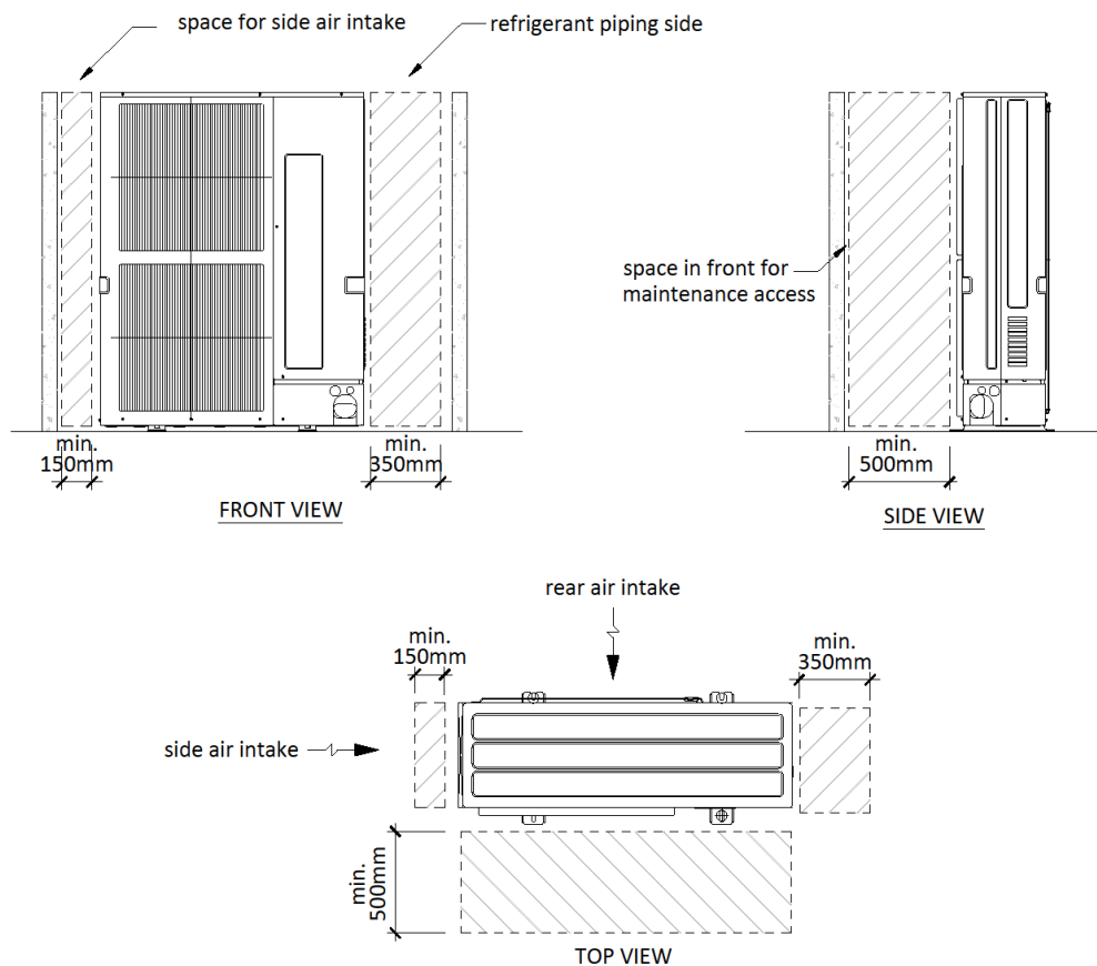
Figure 13: Space requirement for single VRF outdoor installation (side discharge)
