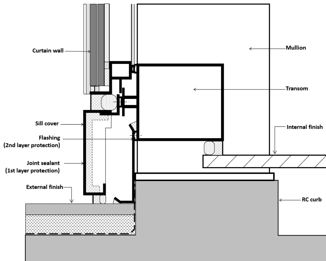
Figure 7: Drawing illustrating double layer protection at bottom flashing, in this case sealant (1 st layer of protection) and flashing (2 nd layer of protection).
