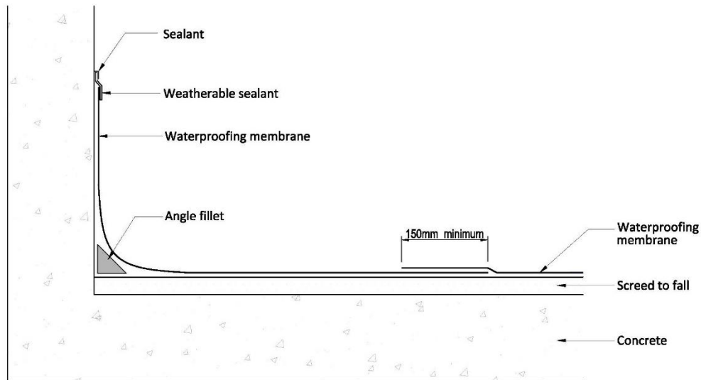
Figure 16: waterproofing termination and overlapping detail
