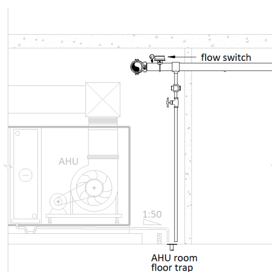
Figure 46: Flow switch drain valve in rooms with floor trap
