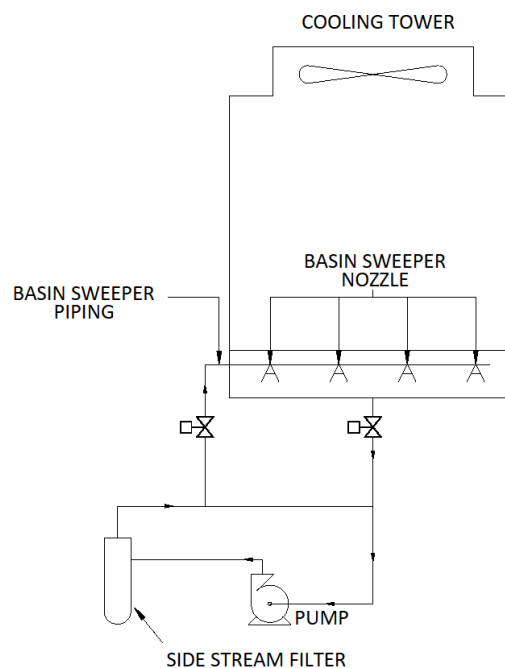
Figure 29: Cooling tower basin sweeper system
