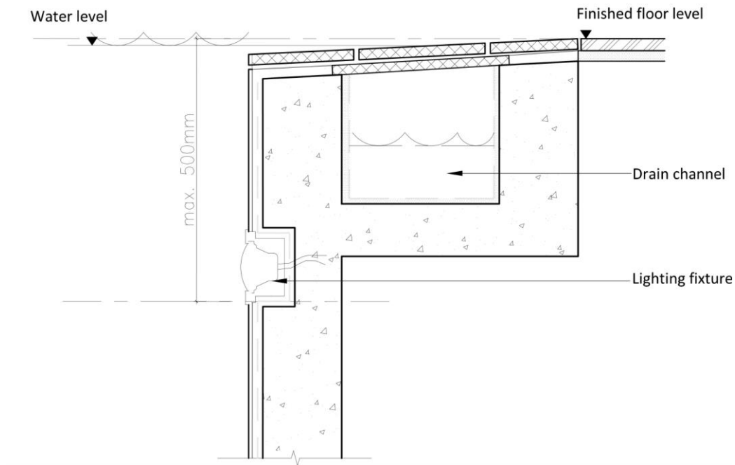
Figure 27 - Section showing the light fixture at accessible distance for repair and maintenance
