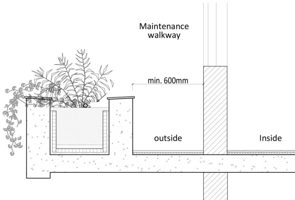
Figure 31 - Planter box with maintenance walkway
