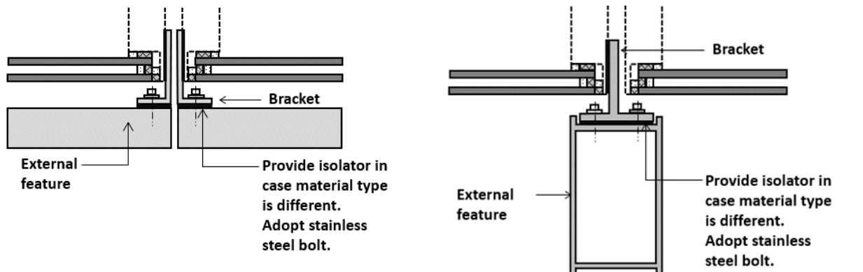
Figure 4: Example – plan drawing (detail) on left and right illustration connection between curtain wall and metal external feature on the exposed face of the façade. Providing metals of similar properties or separator/isolator helps to mitigate risk of bi-metallic corrosion.
