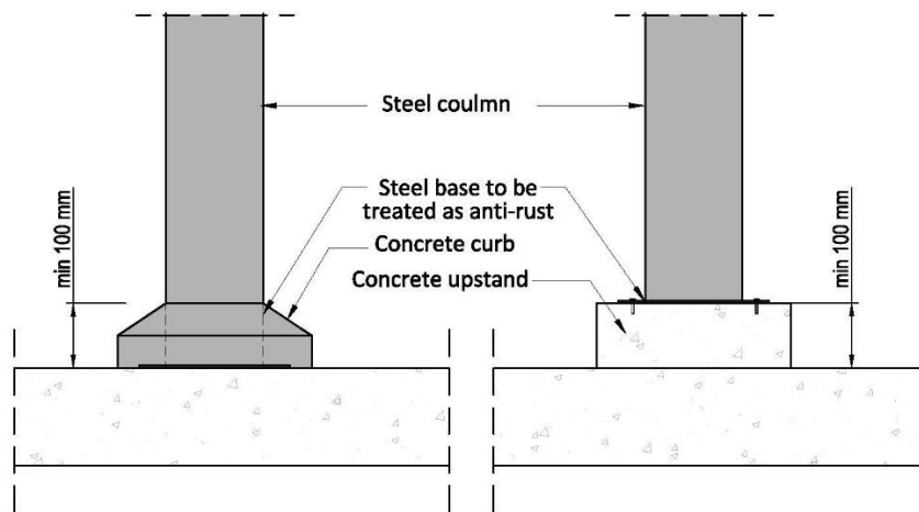
Figure 13: Concrete collar / upstand protection for steel base.
