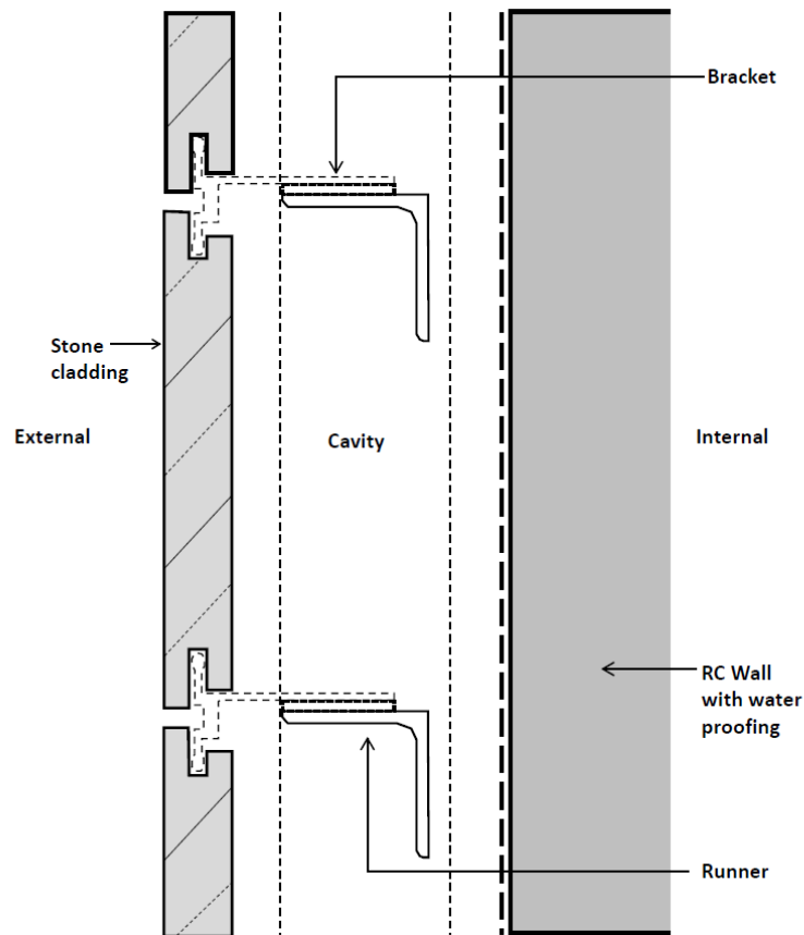
Figure 14: Illustration of mechanically-fixed stone cladding.
