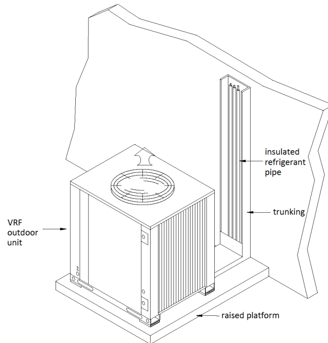
Figure 36: Trucking for refrigerant pipe
