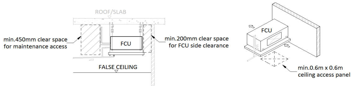
Figure 3718: Typical access provision for FCU
