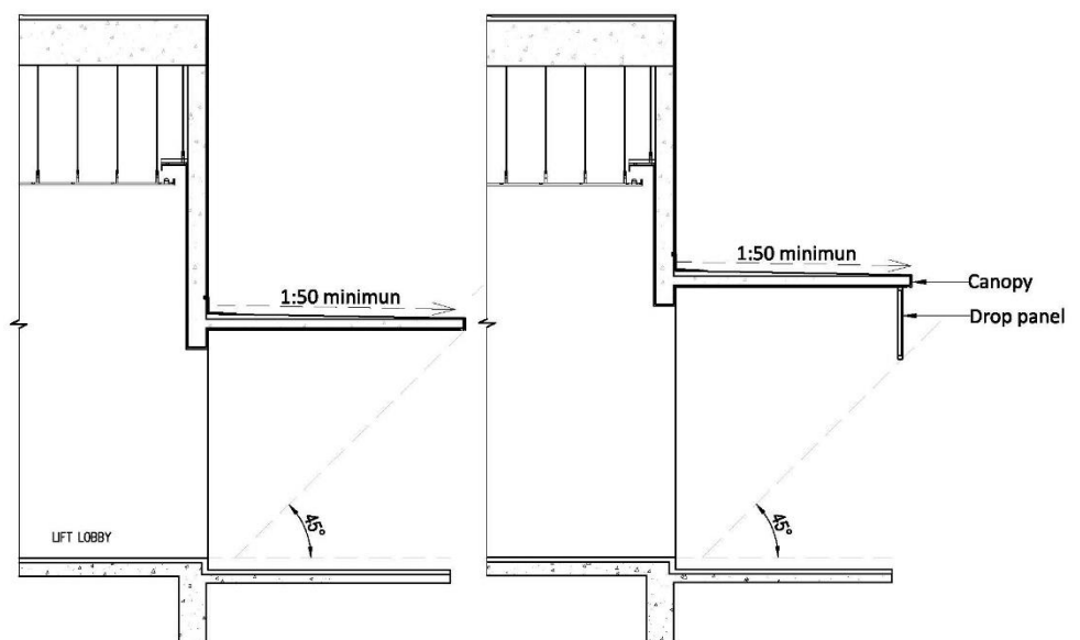
Figure 15: Design of canopy overhang (left), Design of canopy overhang with drop panel (right)
