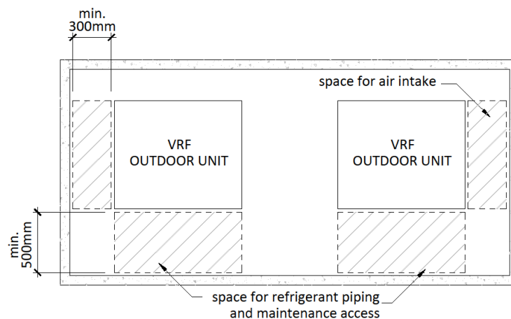
Figure 16:17 Space requirement for VRF outdoor installation (top discharge) – top view
