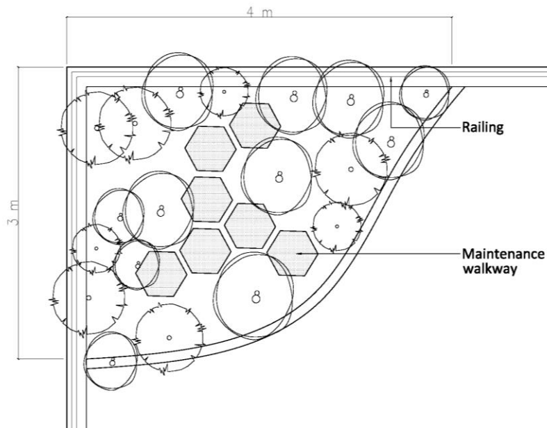
Figure 29 - Maintenance walkway for planter box more than 1.8m wide
