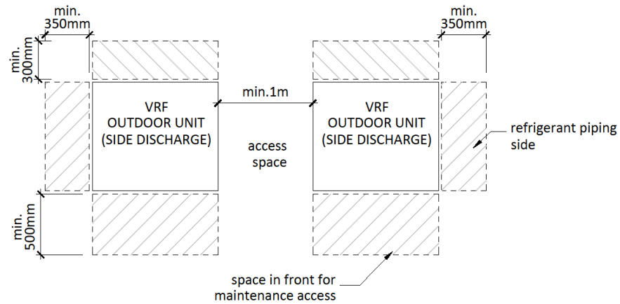
Figure 15: Space requirement for collective VRF outdoor unit (side discharge) – top view
