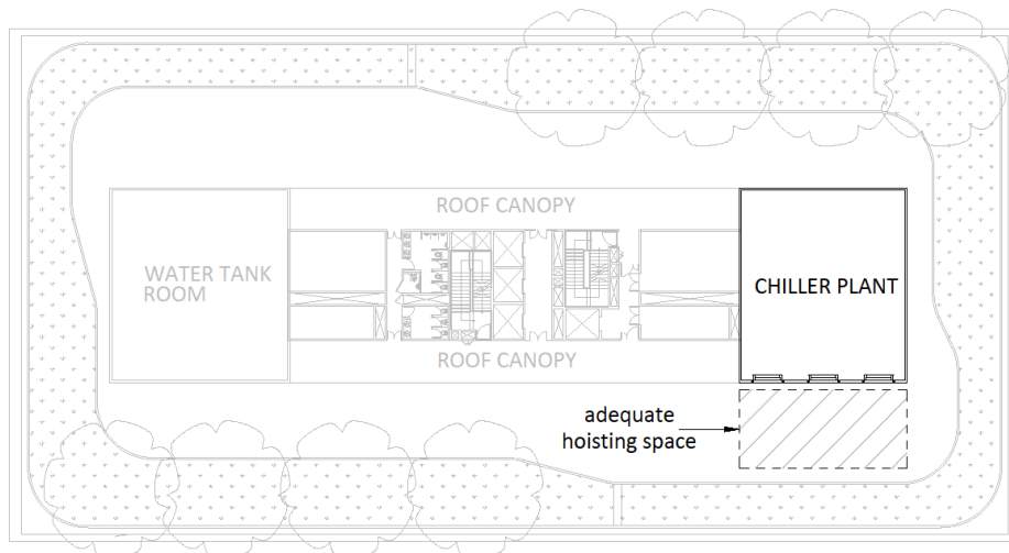
Figure 82: Rooftop chiller plant with operable opening and adequate hoisting space
