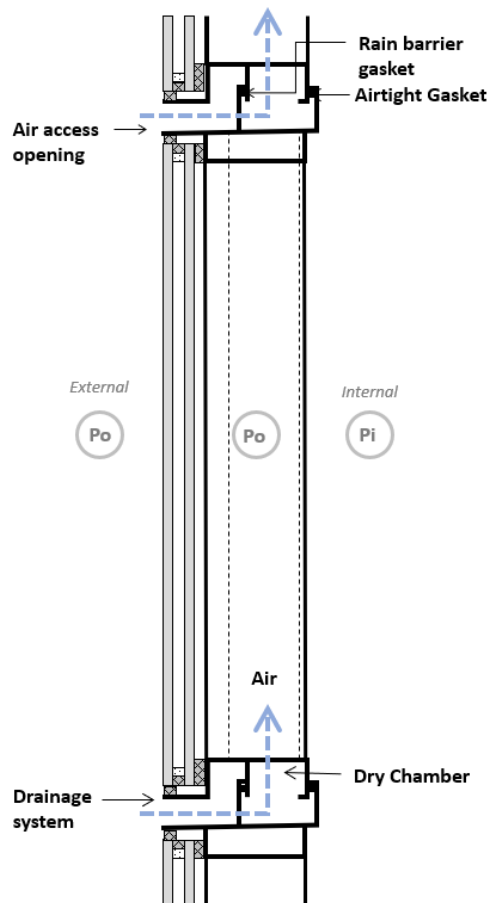
Figure 8: Drawing illustrating pressure equalised system.
