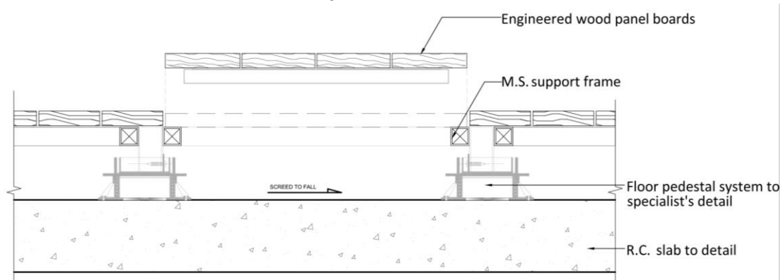
Figure 28 - Typical section showing demountable fixture deck system
