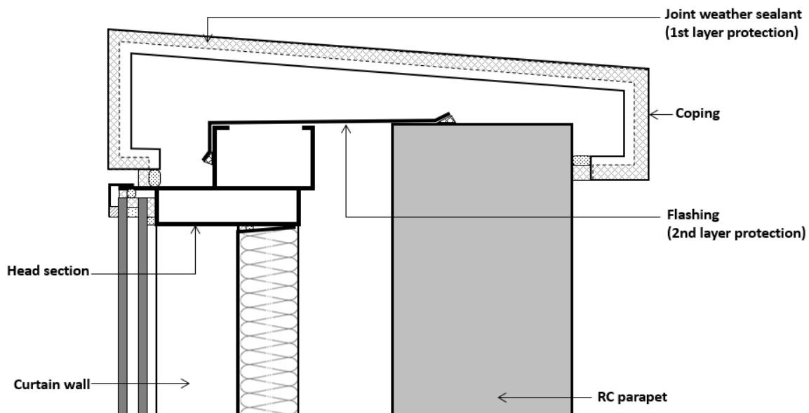
Figure 6: Drawing illustrating double layer protection at façade coping, in this case sealant (1 st layer of protection) and flashing (2 nd layer of protection).
