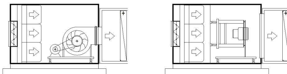
Figure 201: Conventional (left) and Direct Drive Fan system (right)
