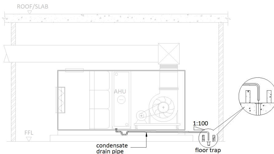
Figure 38: Typical AHU condensate drain termination
