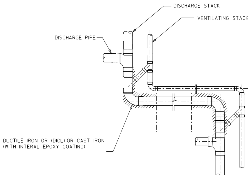
Figure 32: Hubless elbows for sanitary stacks with horizontal transfers 29
