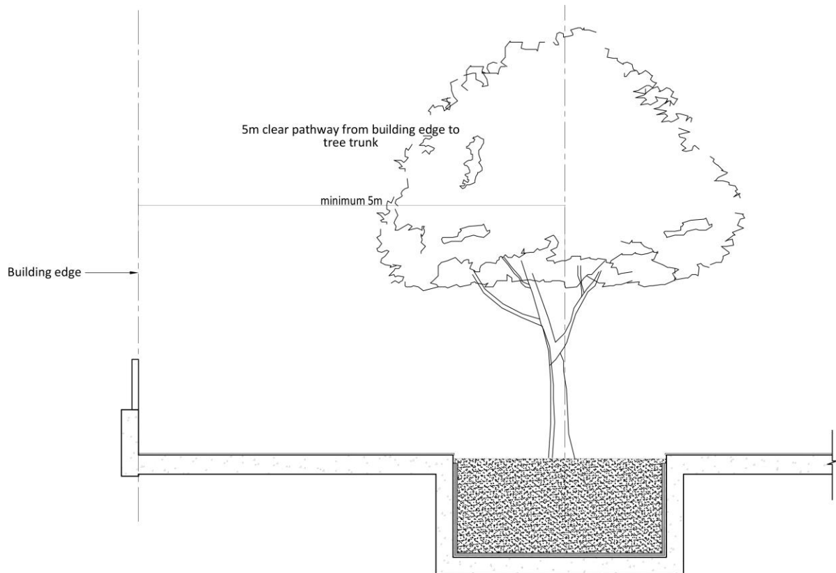
Figure 44- Typical section showing buffer zone required for trees
