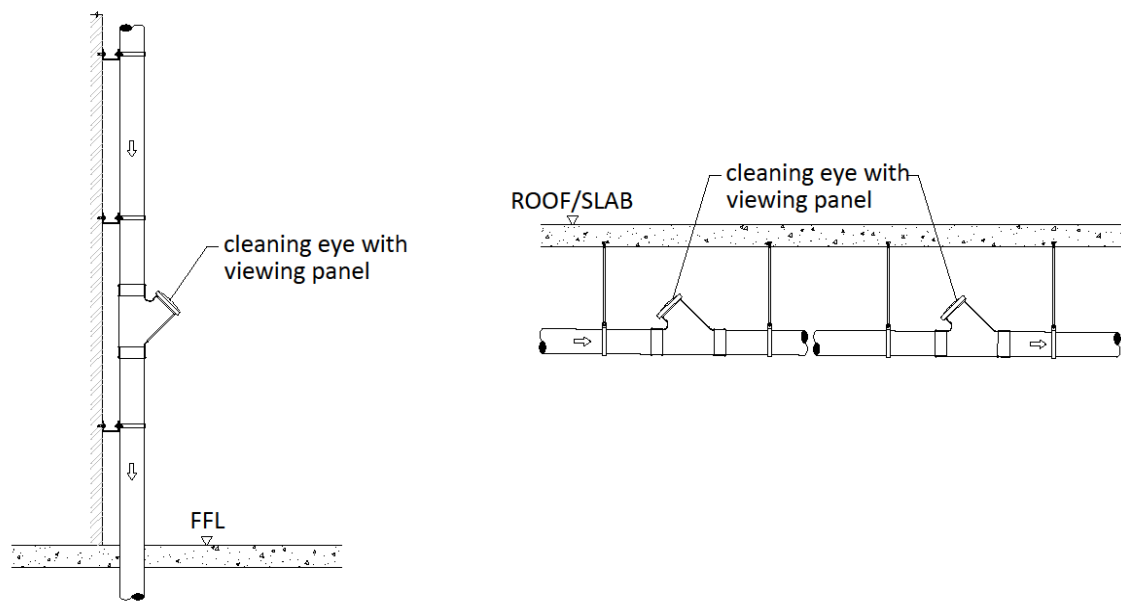
Figure 31: Sanitary pipe with cleaning eye that equipped with viewing panel
