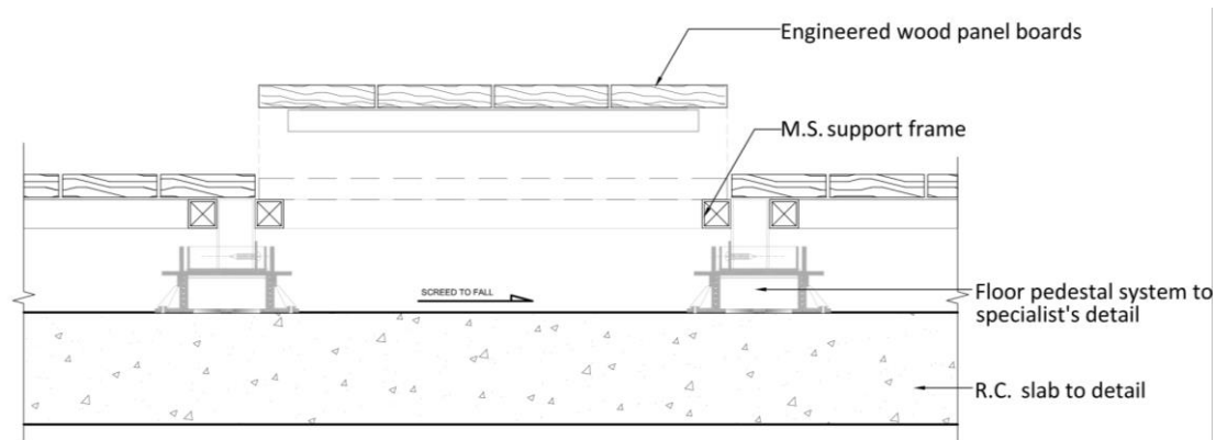
Figure 42- Typical section showing demountable fixture deck system
