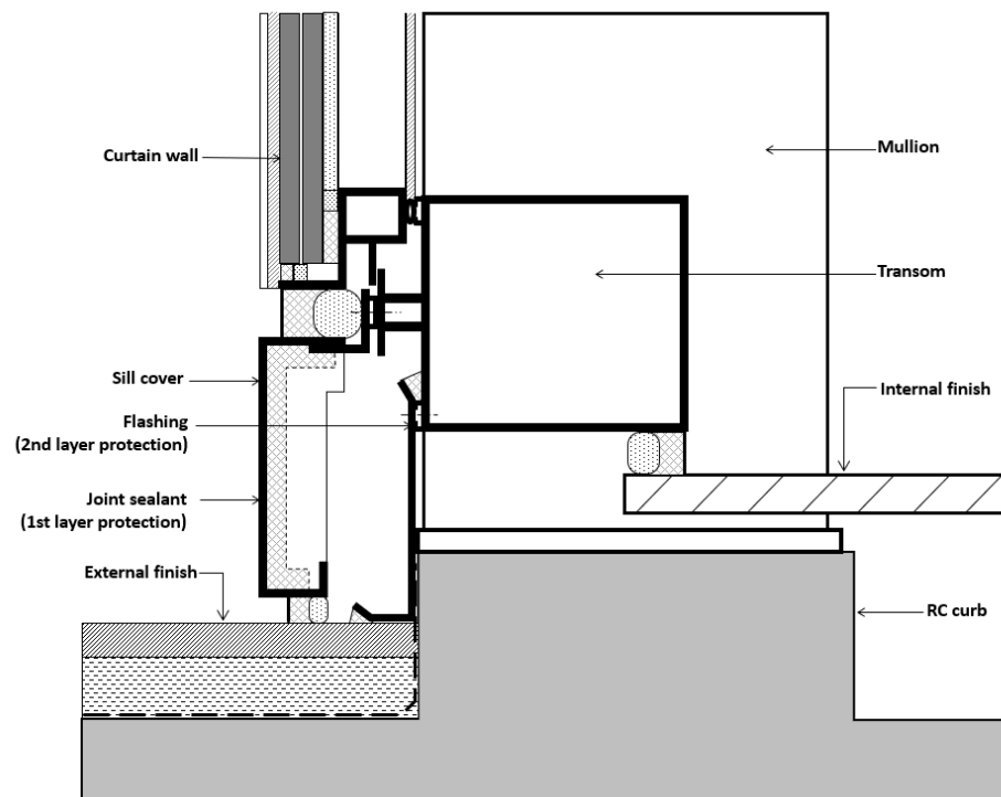
Figure 15: Drawing illustrating double layer protection at bottom flashing, in this case sealant (1 st layer of protection) and flashing (2 nd layer of protection).
