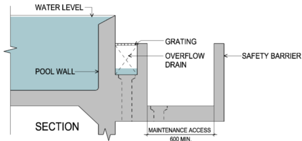
Figure 45- Typical section showing provision of overflow drain and maintenance access
