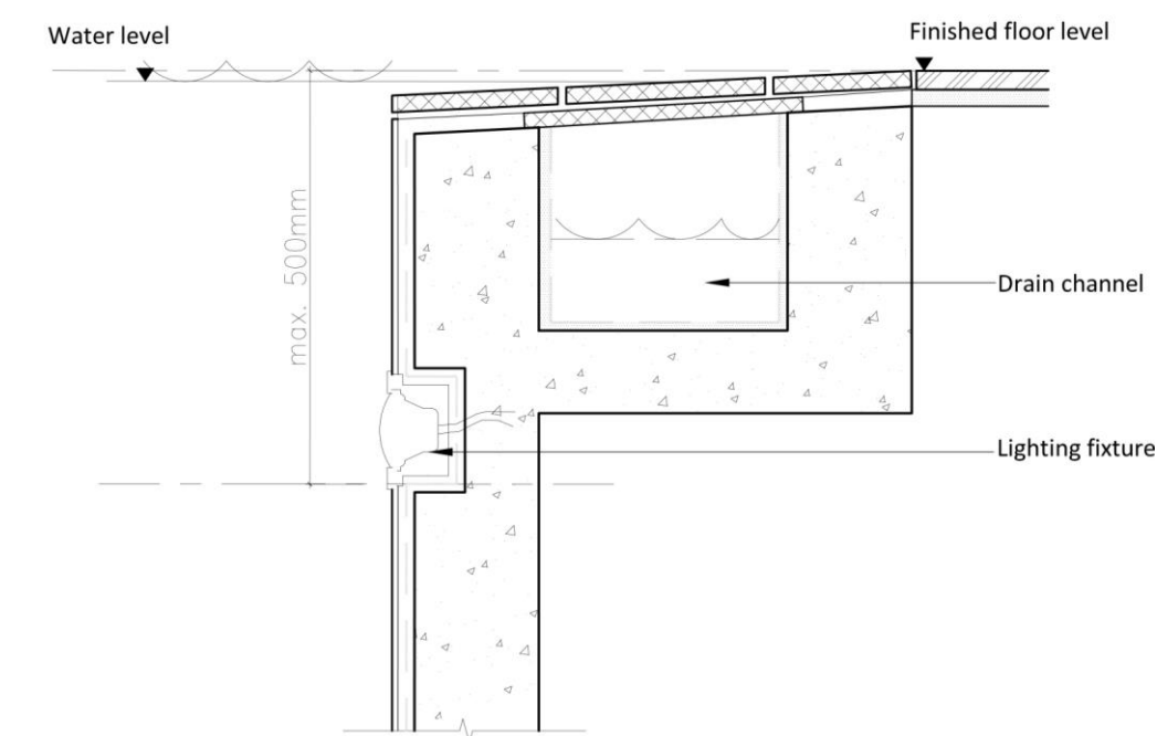
Figure 41- Section showing the light fixture at accessible distance for repair and maintenance
