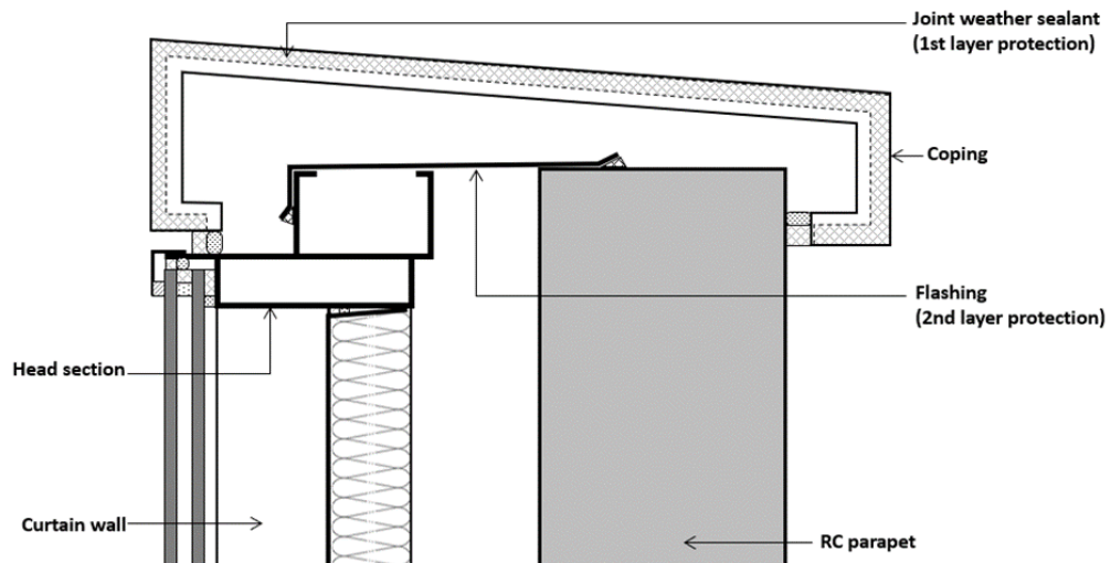
Figure 14: Drawing illustrating double layer protection at façade coping, in this case sealant (1 st layer of protection) and flashing (2 nd layer of protection).
