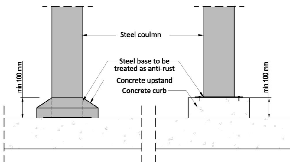
Figure 46- Concrete upstand protection for steel base
