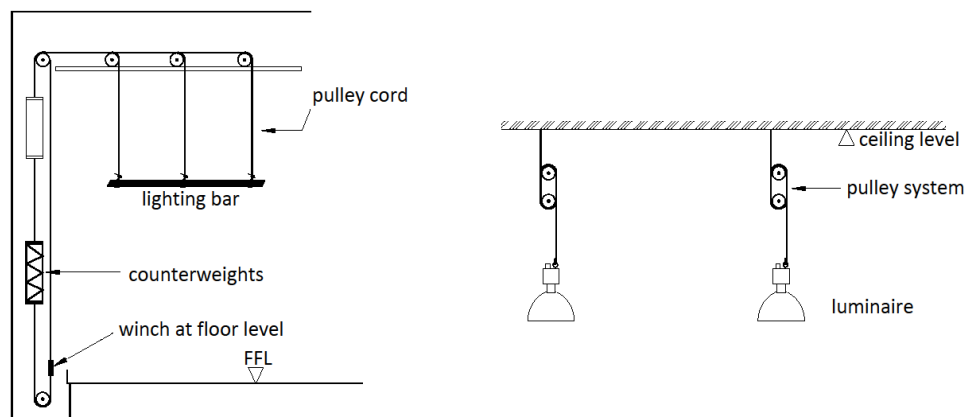
Figure 35: Group pulley system (left) and single pulley system (right)
