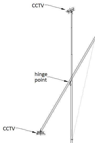
Figure 38: CCTV with foldable pole and arm
