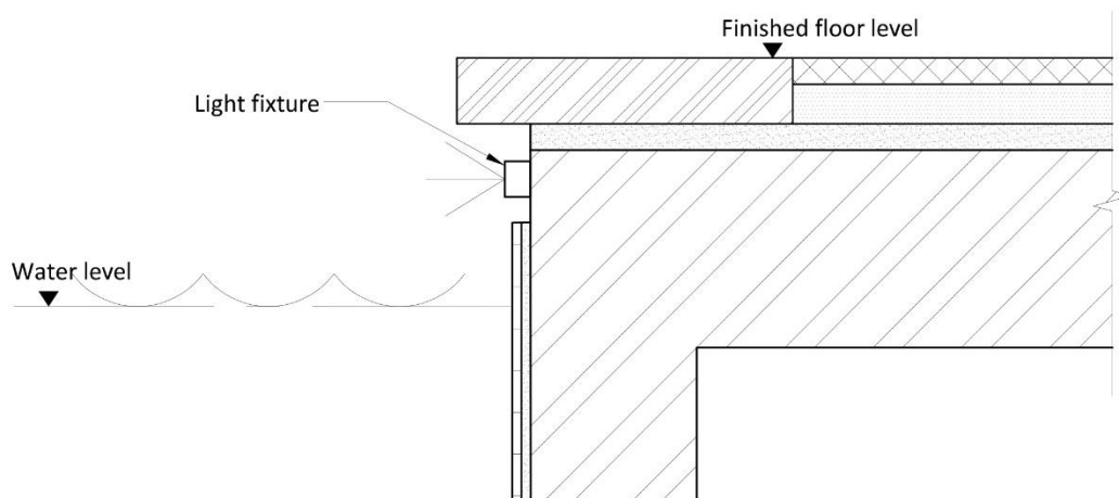
Figure 40- Example of lighting system located above the water
