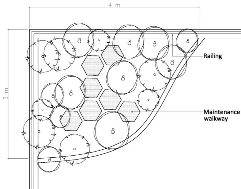
Figure 43- Maintenance walkway for planter box more than 1.8m wide
