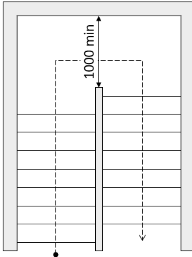
Figure E.3.5.3(a) Measurement of landing width
