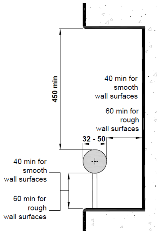
Figure E.3.6.4(a) – Handrail in Recess
