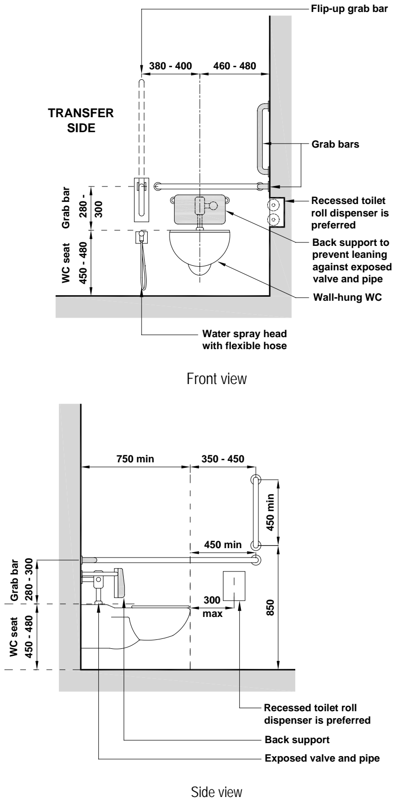
(b) Wall-hung water closet with exposed pipe and valve
