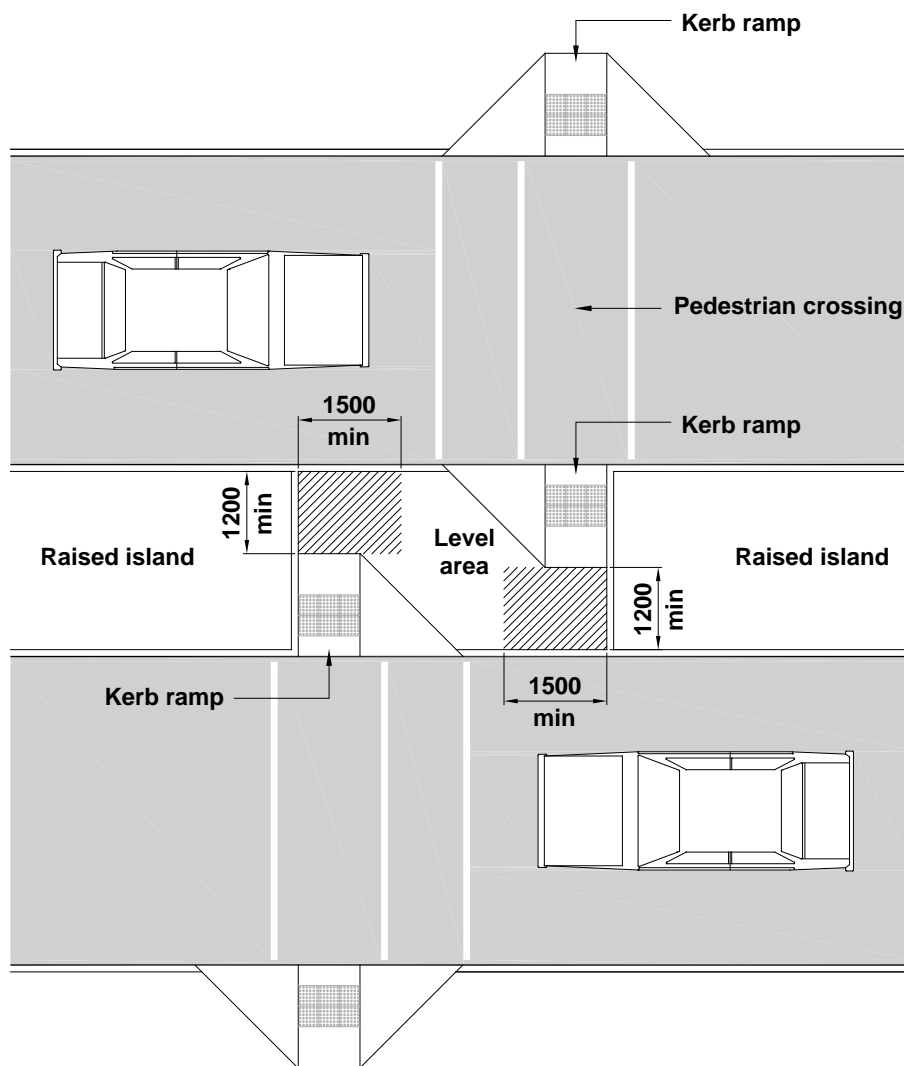
Figure 12 Kerb Ramps Location on Island
