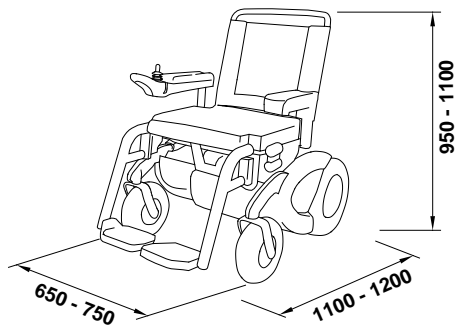
(b) Example of an electric wheelchair
