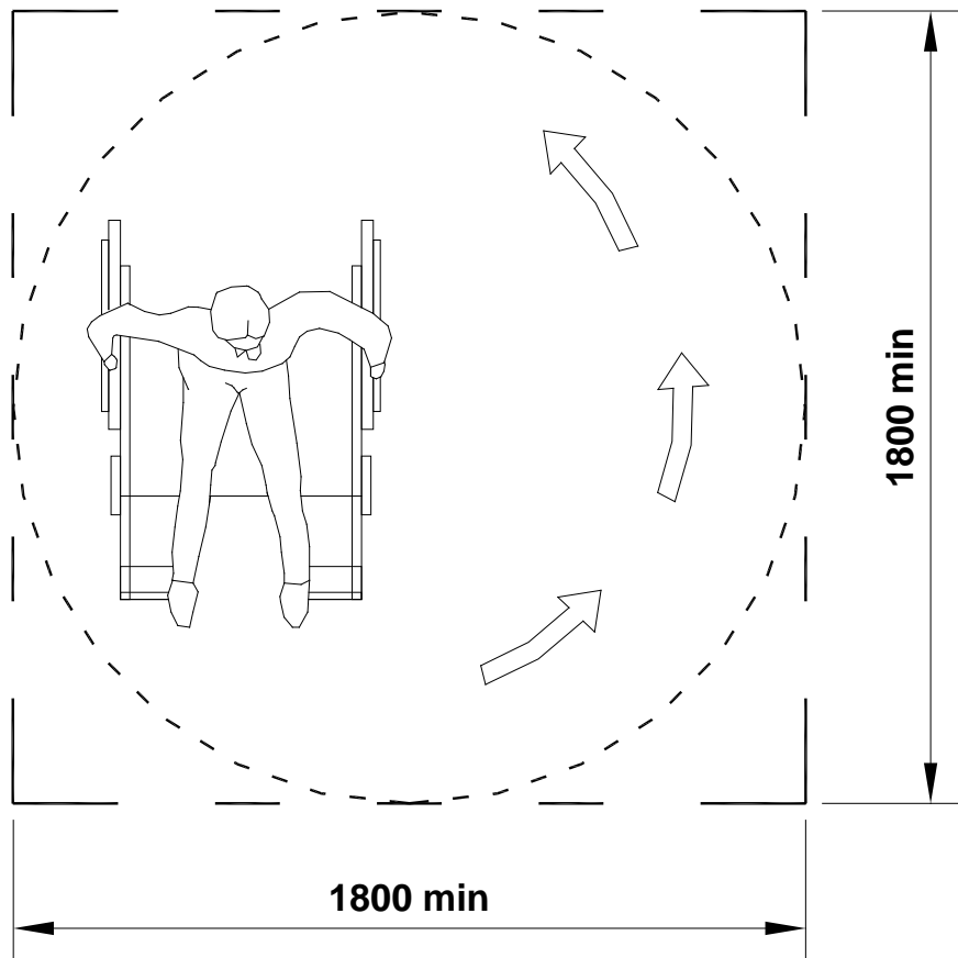
Figure 81 Wheelchair Space Allowances: Minimum Clear Turning Space
