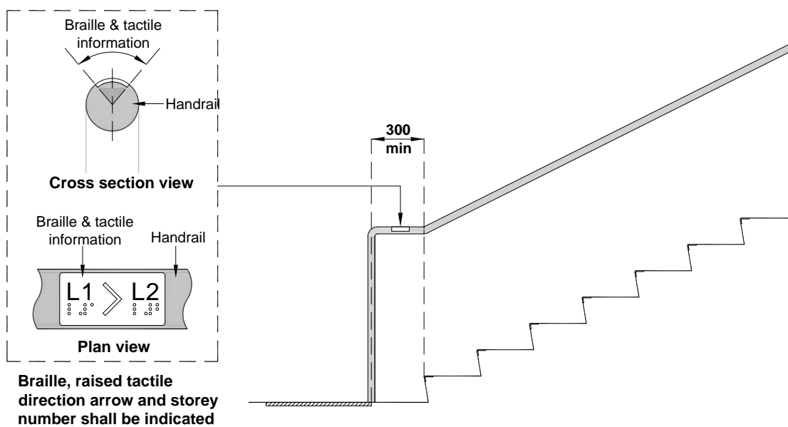
(b) Handrail extension at Bottom of Stairs
