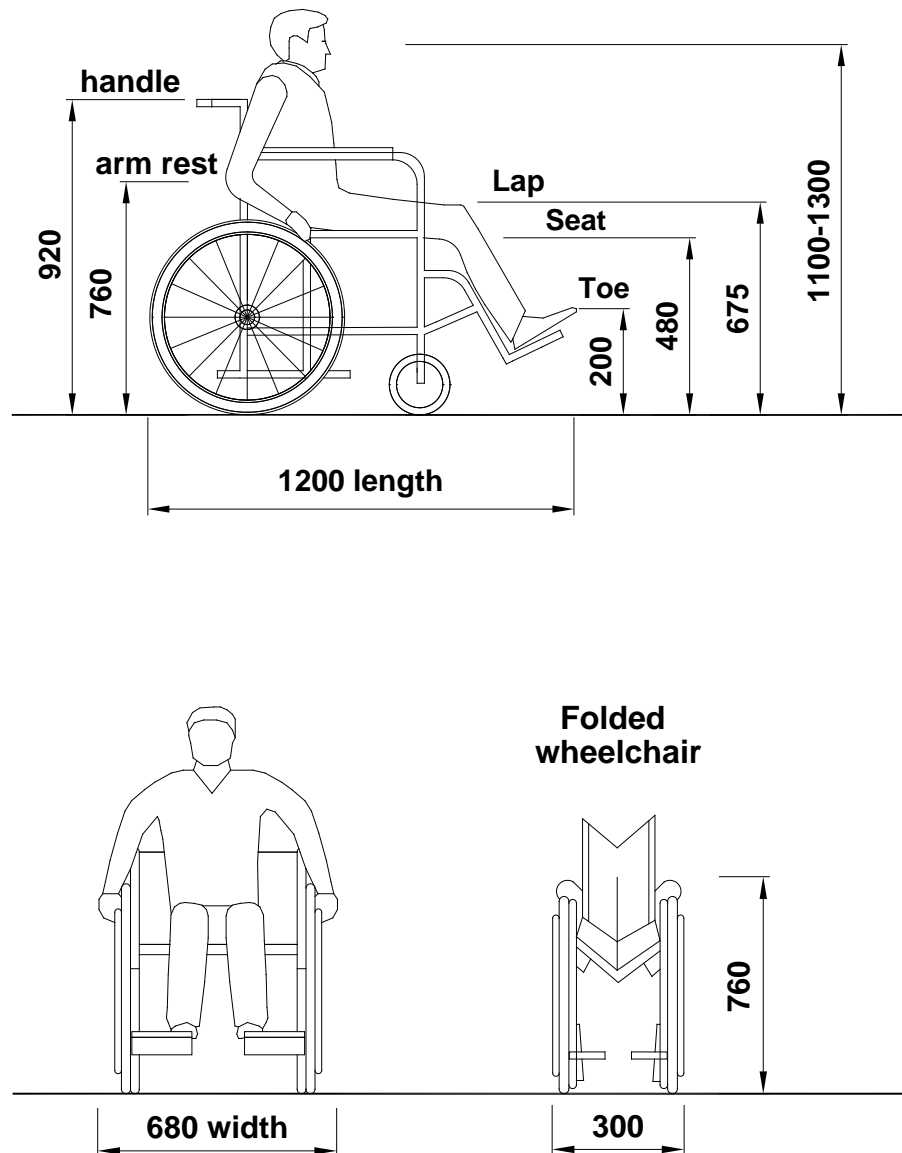
Figure 82 Typical Dimensions of Wheelchairs Commonly Used by Adults
