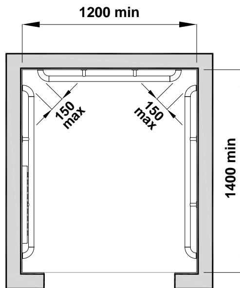
Figure 40 Grab Bars in Lift Cars
