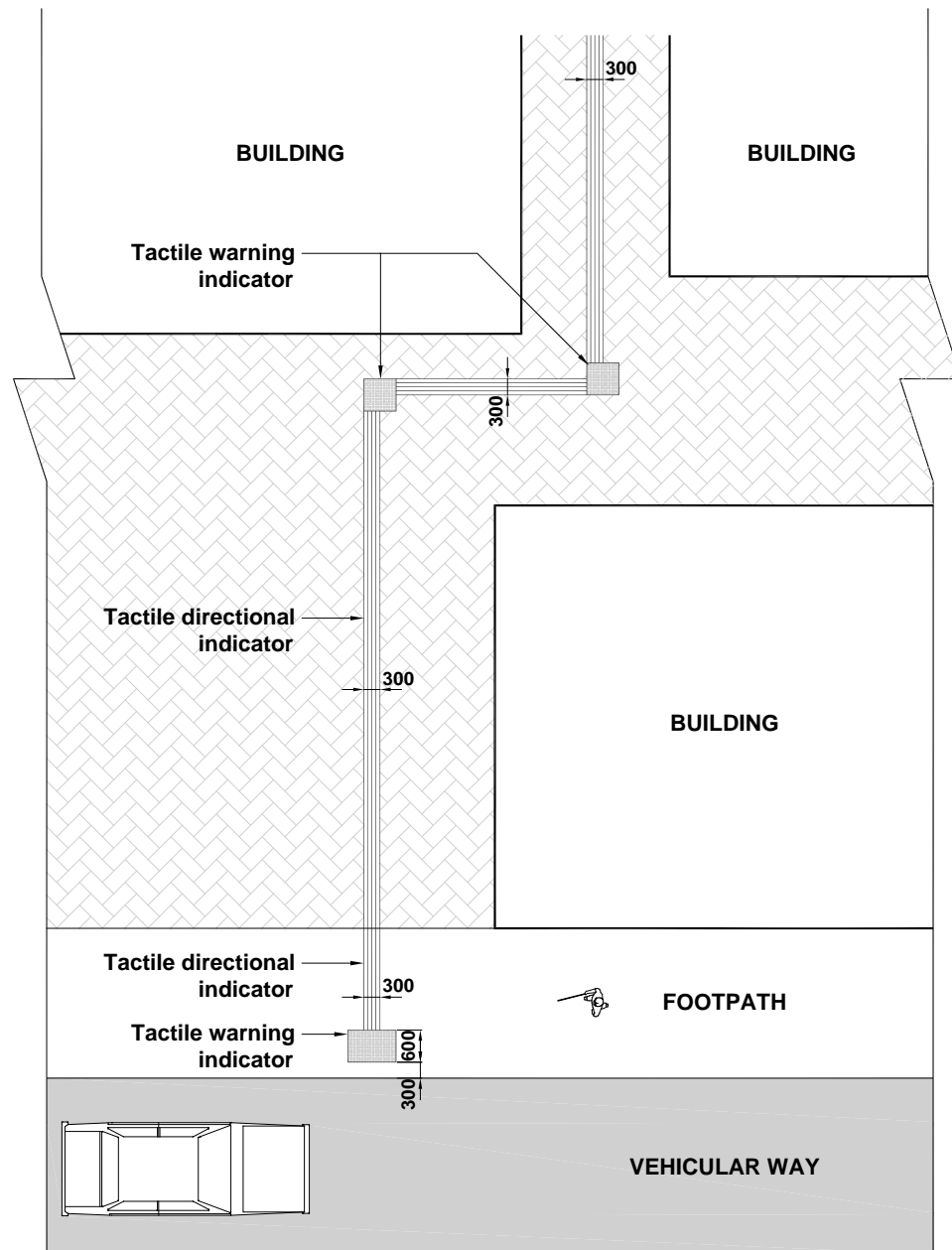
Figure D10 Tactile Guidance Strips
