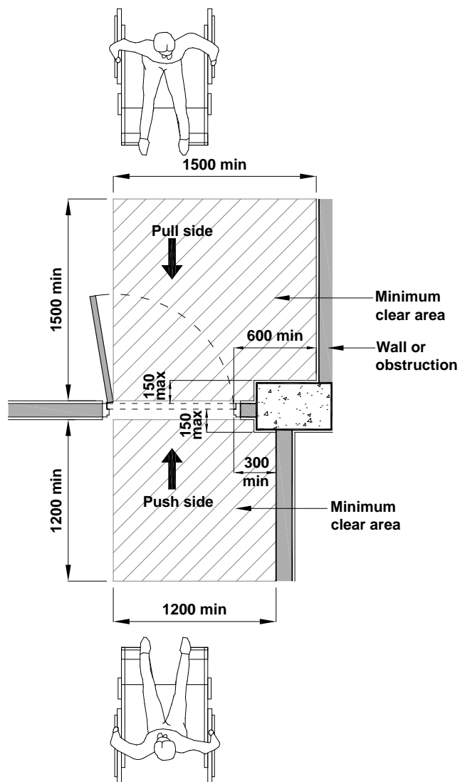
Figure 26 Minimum Doorway Manoeuvring Space at Leading Edge of Door Leaf
