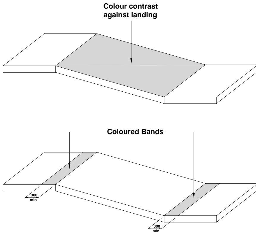
(a) Use of colour contrast or coloured bands for rises from 15 to 200 mm
