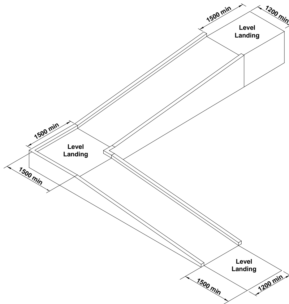
Figure 34 Level Landings and Edge Protection
