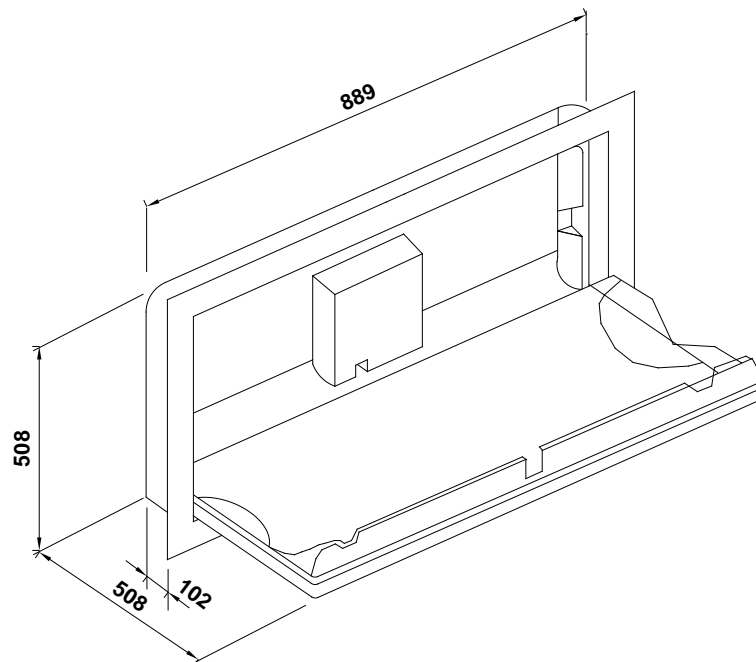
Figure A7 Example of Flap-type Diaper Changing Station
