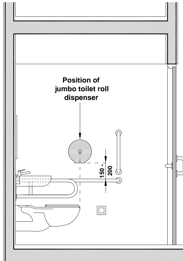
Figure 49 Location of Jumbo Toilet Roll Dispenser
