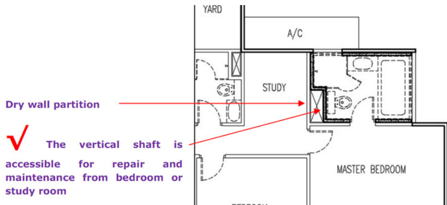
Figure 2 – Example of a layout of a prefabricated bathroom unit with a services shaft that is accessible for future repairs and maintenance
