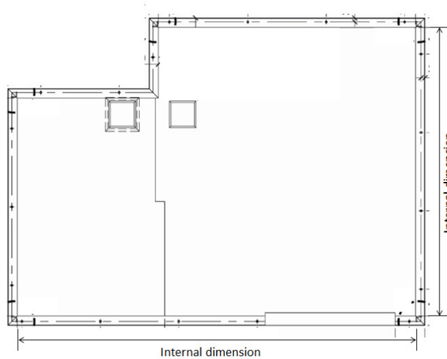
Figure 1 – Plan of a prefabricated bathroom unit and its internal dimensions
