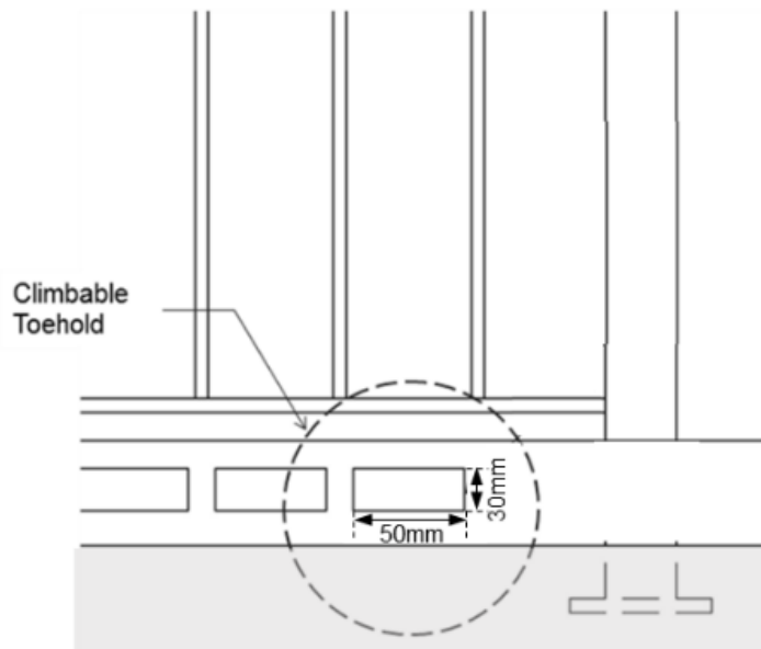
Front View of Railing
