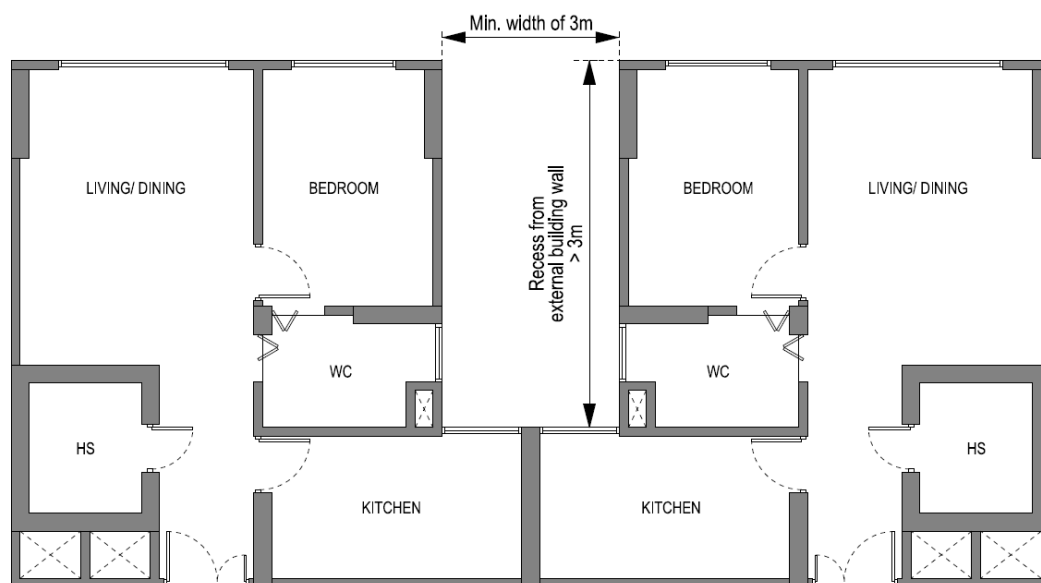
Figure G.3.2.2(b) – Recessed Void Dimension
