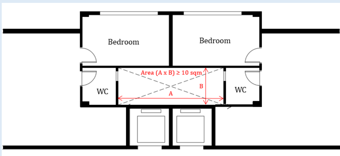
Figure G—XVIII: Calculations of air wells and voids
