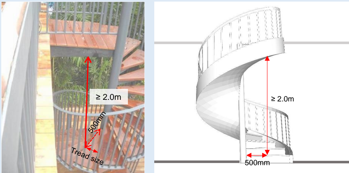
Figure E—IV: Measurement of headroom for a spiral staircase
