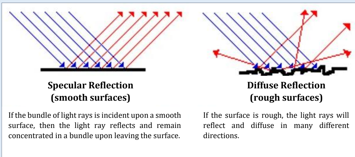
Figure P—1: Comparison of specular and diffuse reflection
