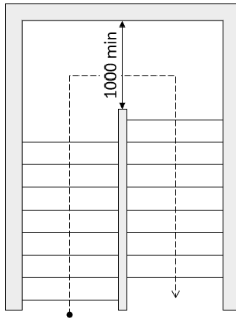
Figure E.3.5.3(a) Measurement of landing width
