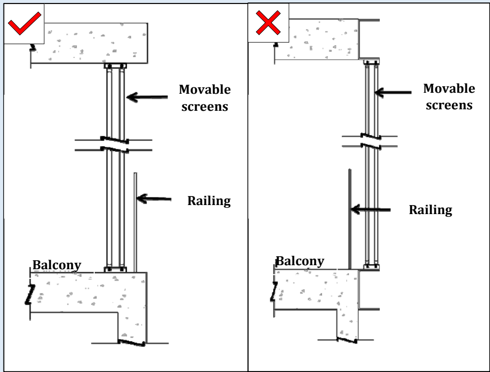
Figure A3-1: Exterior Movable Balcony Screens should be on interior of building/parapet wall
