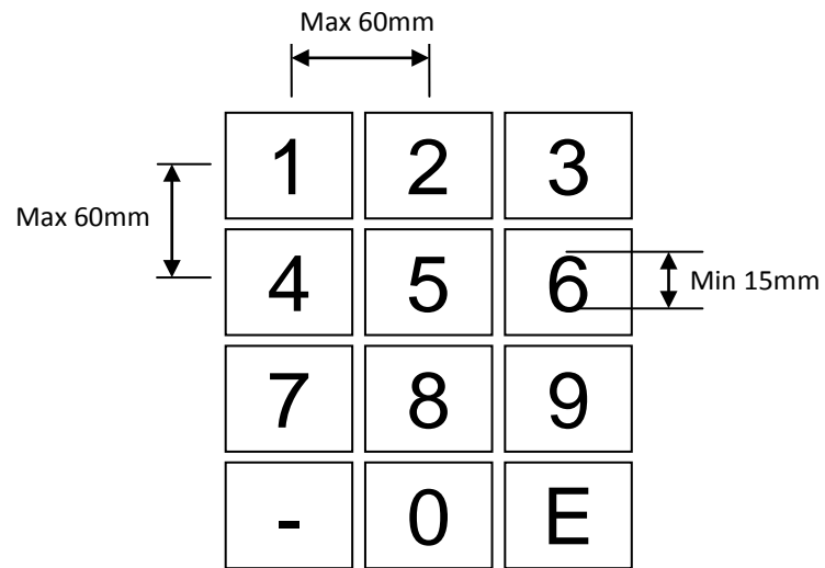
Figure G1 Keypad Buttons
