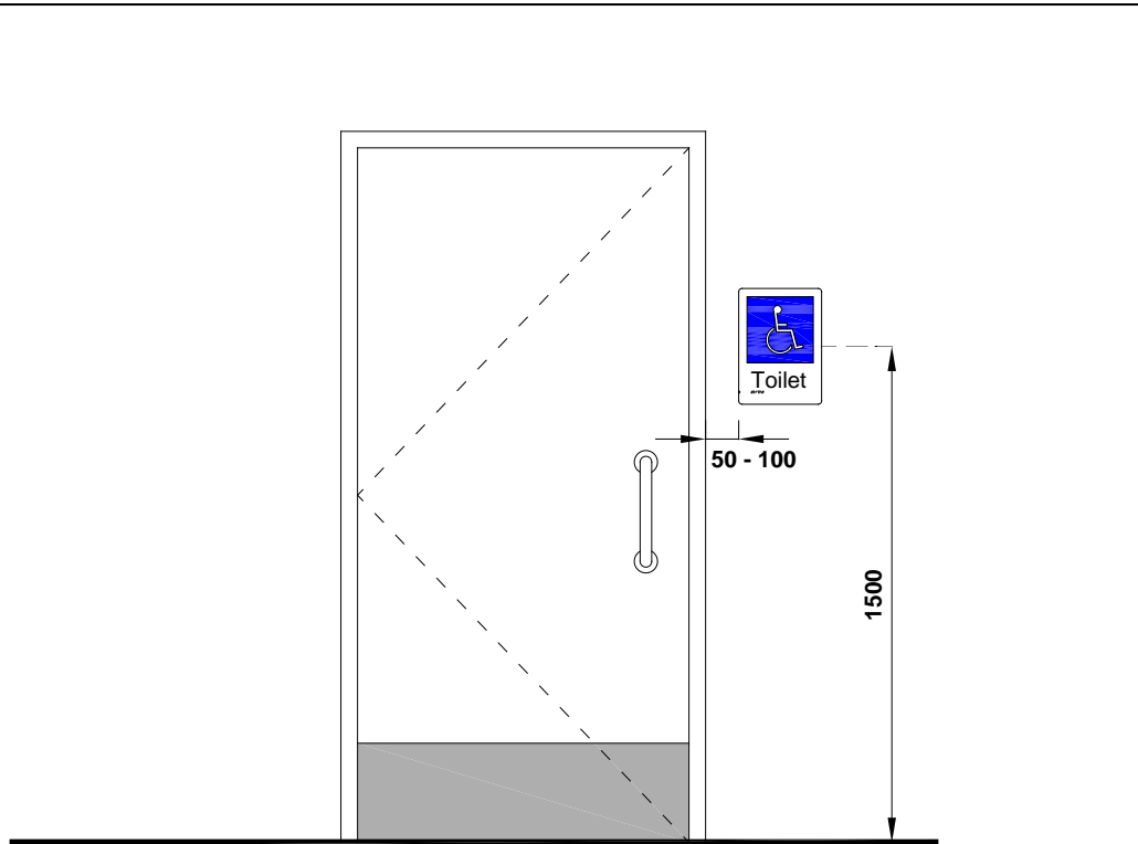
(a) Example of Signage at Accessible Individual Washroom
