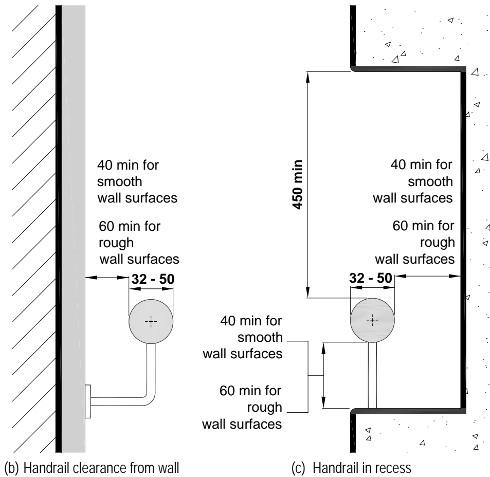
Figure 38 Handrails
