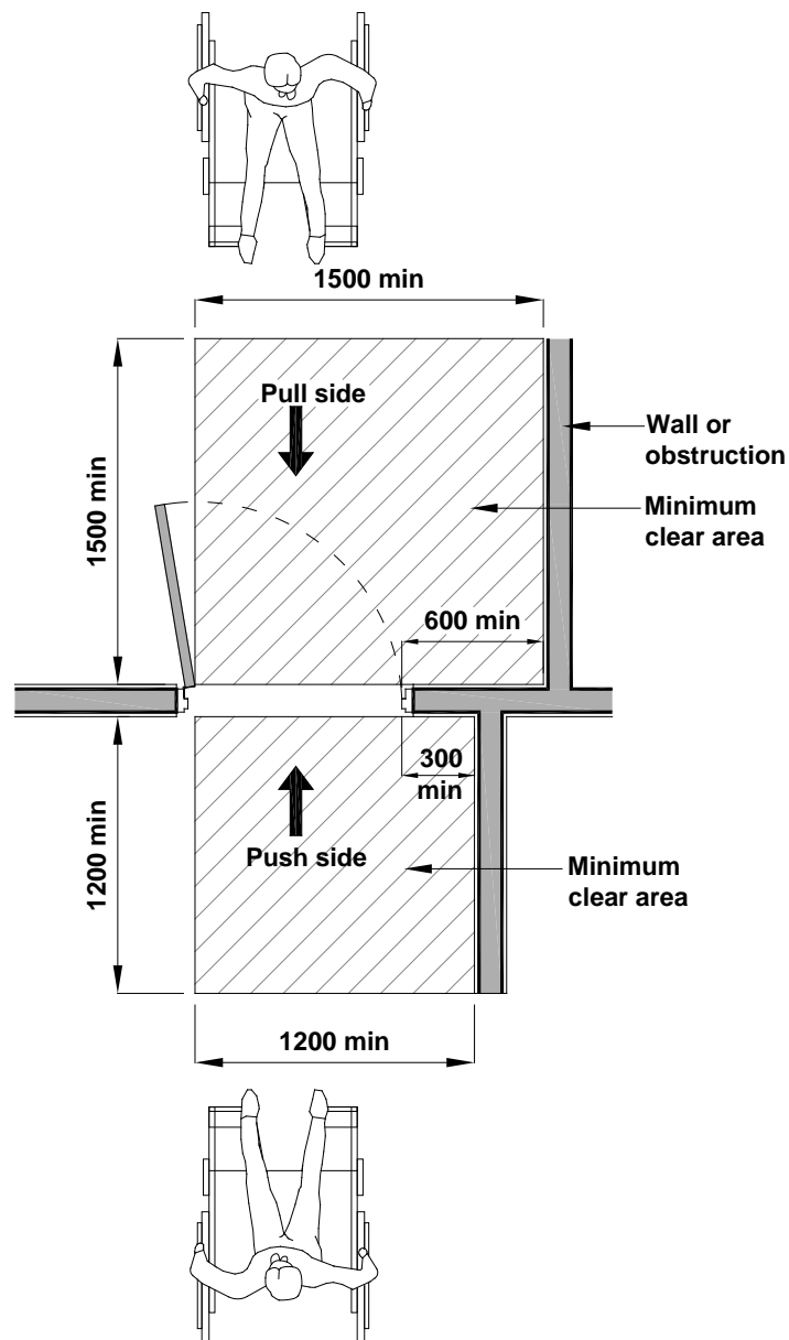
Figure 24 Minimum Doorway Manoeuvring Space
