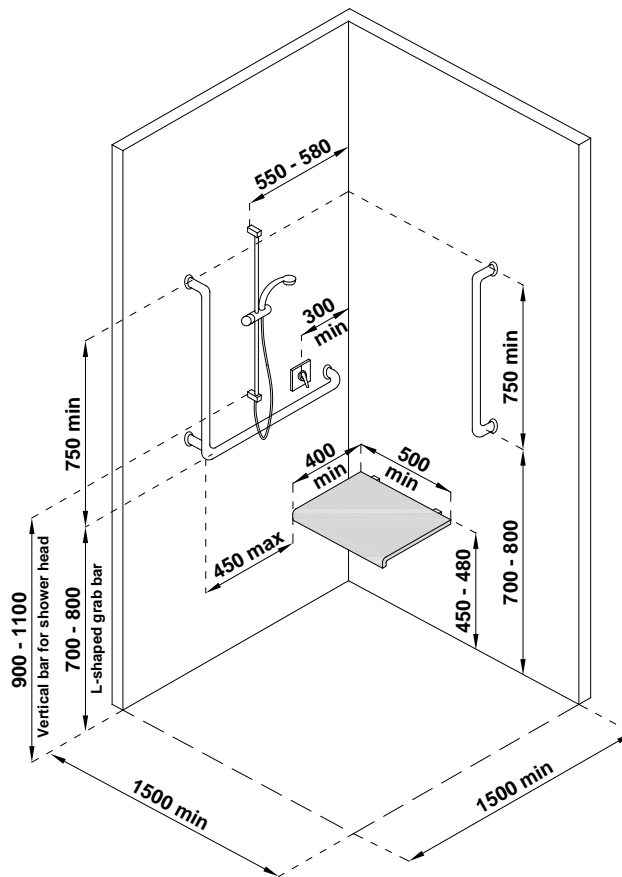
(b) Isometric view of roll-in shower stall
