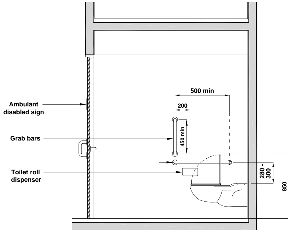
(c) Side view of ambulant disabled water closet compartment
